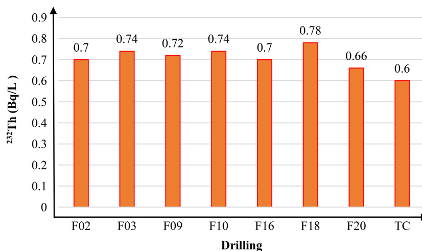
Figure 9. Specific activities of ^{232}\text{Th} in drilling water samples.
