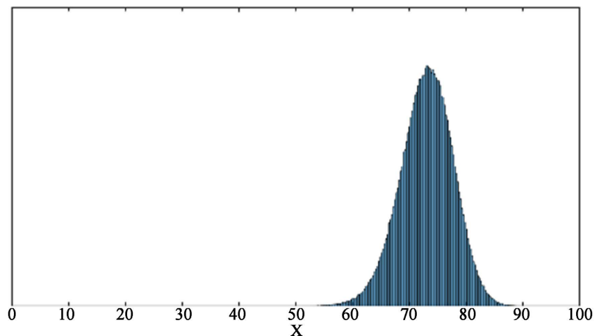
Figure 7. Geometric average X = (X_1 X_2 \dots X_N)^{1/N} .
