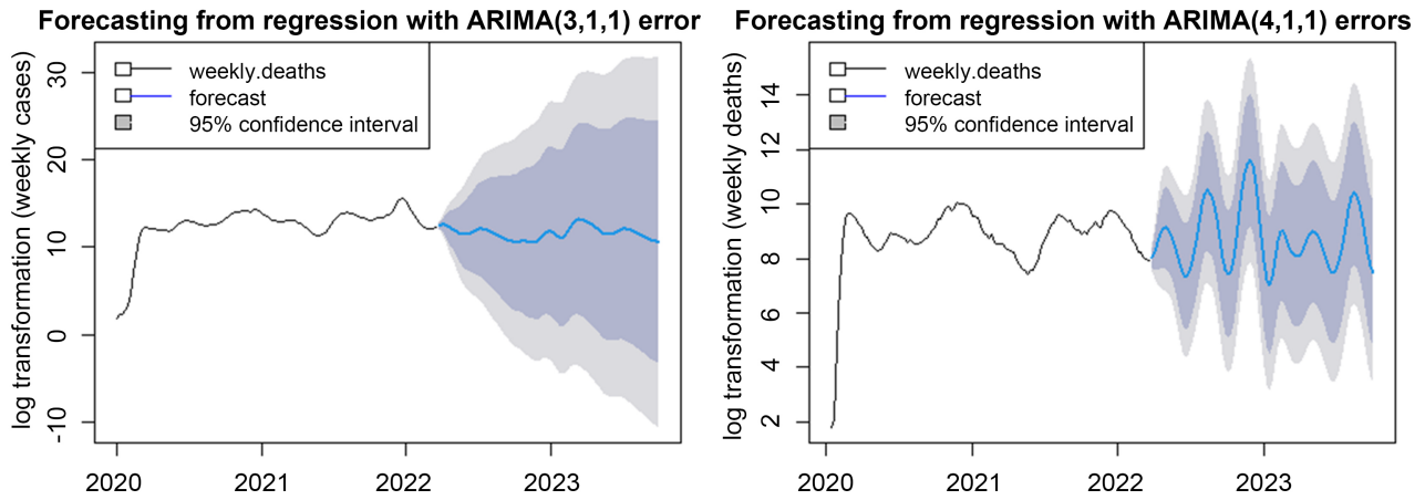
Figure 1. Forecasting results.
