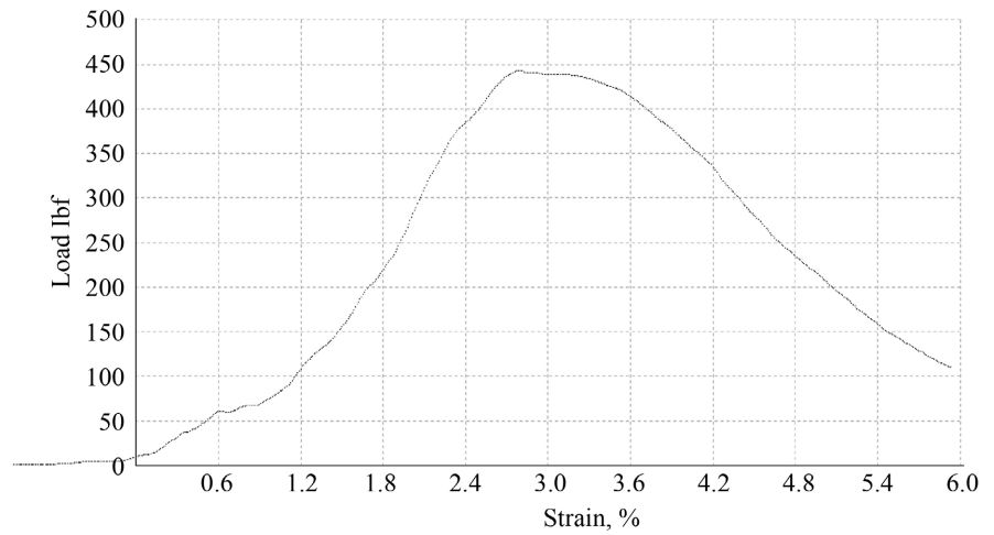
Figure 12. Stress-strain curve for L-F.
