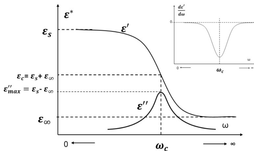
Figure 6. The complex dielectric permittivity ( \epsilon^*(\omega) ) in Debye scheme. The derivative of the real part ( \frac{d\epsilon'}{d\omega} ) has a minimum in \omega_c . It is shown in the insert.
