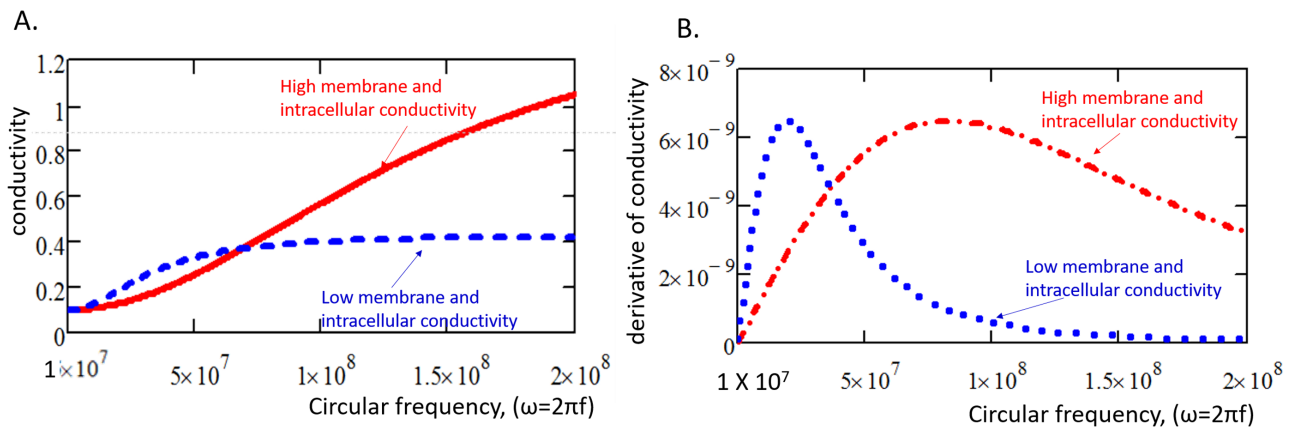
Figure 7. The conductivity vs. circular frequency \omega = 2\pi f of a unit cube of the tissue at the low ( \sigma_2 = \frac{1}{3} S/m) and high ( \sigma_2 = 1 S/m) membrane and intracellular resistivity, ( C = 10^{-8} F; \sigma_1 = 0.1 S/m). (A) The conductivity; (B) The derivative (slope) of the conductivity function. The numeration of conductivity corresponds to Figure 1(B) .
