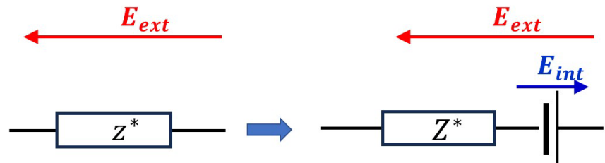
Figure 9. Model of the effect of the Nernst-Planck principle on a material having z^* impedance developing Z^* + E_{int} by forming Nernst-Planck space charge. The non-perfect dielectric material develops an internal electric field by a double layer influenced by the external electric field. The newly formed electric field can be modelled by an additional opposite field caused by the internal rearrangement of charges.
