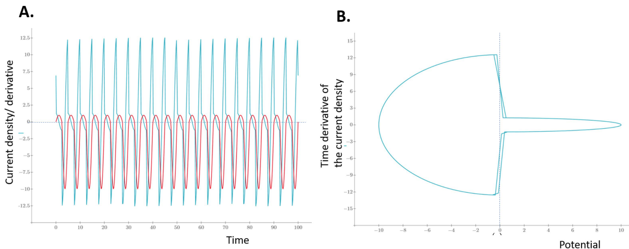
Figure 13. The time-derivative of the current density shows non-linear behavior. (A) The current density and its derivative. (B) The time derivative of current density has hysteresis by the changing potential.
