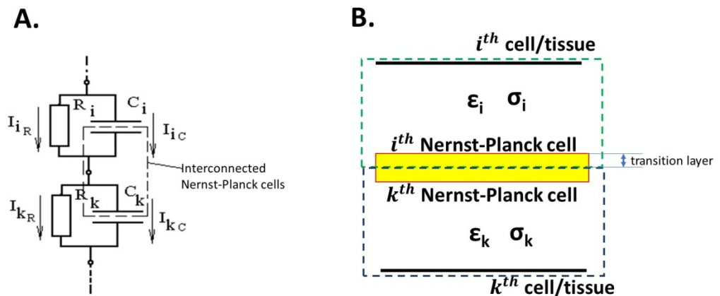
Figure 10. Transition layer schematic of the i^{th} Nernst-Planck cell of the corrected model.
