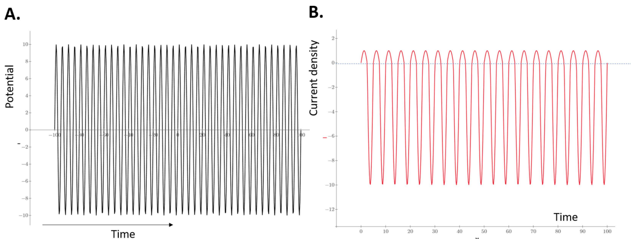
Figure 12. Nernst-Plank cell characteristics. (A) The harmonic external signal. (B) The current density having C_1/C_2 = 10 . The rectification modifies the time-dependence.
