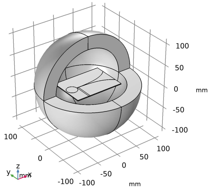
Figure 1. Vidalvi antenna model.
