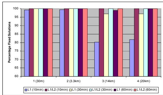
Fig. 15 Availability of Ambiguity Fixed Positions (Post Processing)
