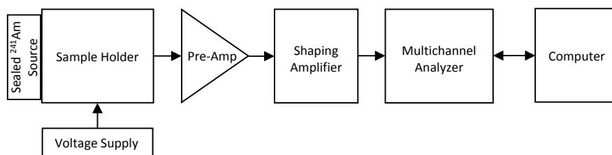
Figure 3. Schematic diagram of the detector repose measurement system (not drawn to scale).
