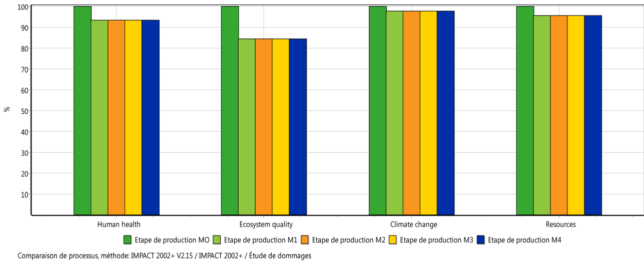
Figure 17. LCA2 of mortars.
