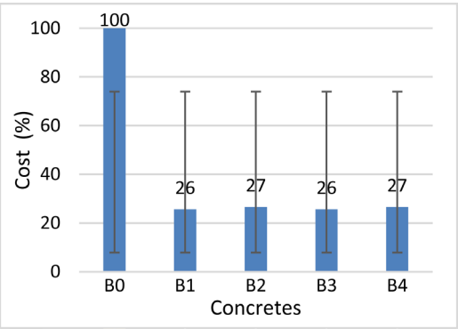
Figure 23. Influence of distance from quarry 3 on the cost of concrete.
