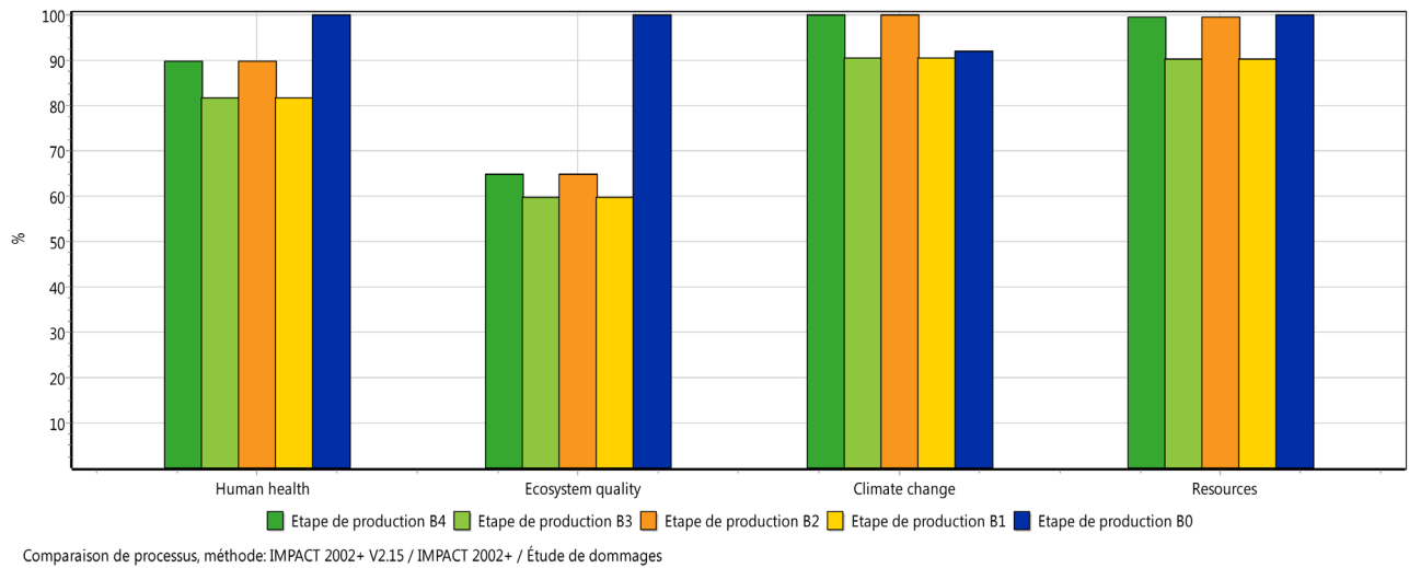
Figure 13. LCA3 for concrete.
