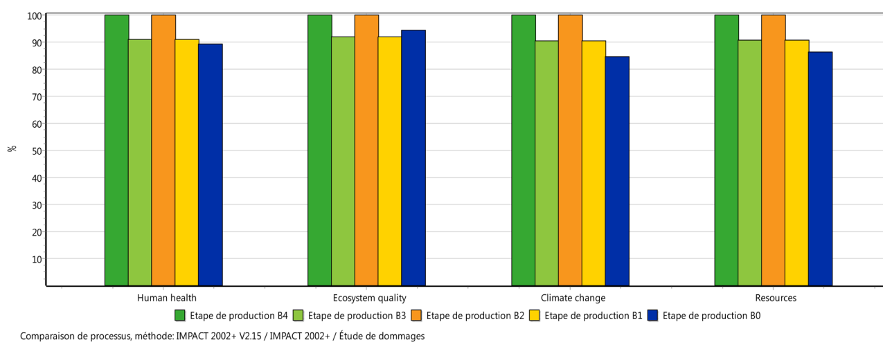
Figure 15. LCA5 for concrete.
