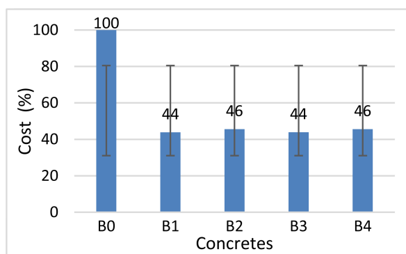
Figure 22. Influence of distance from quarry 2 on concrete costs.
