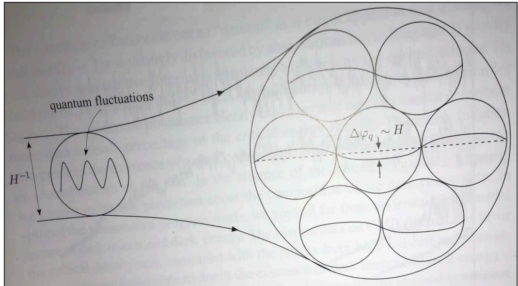
Figure 3. Which is from reference [11] [15].
