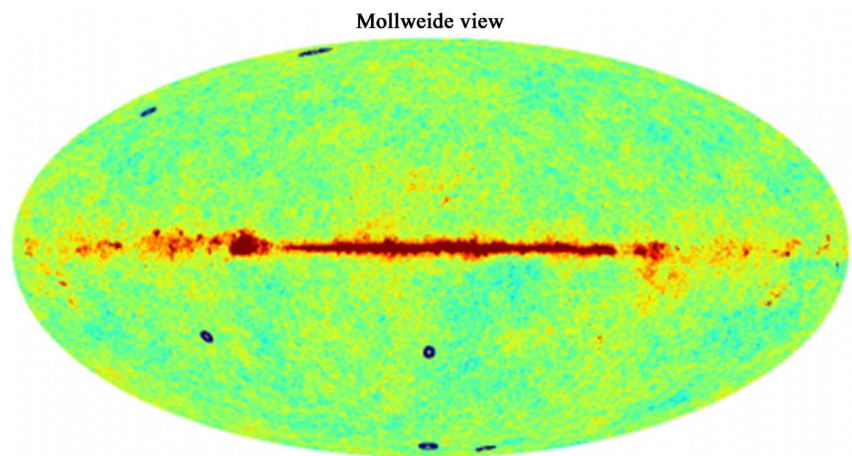
Figure 4. Penrose addendum to CMBR including pre Big bang contributions.
