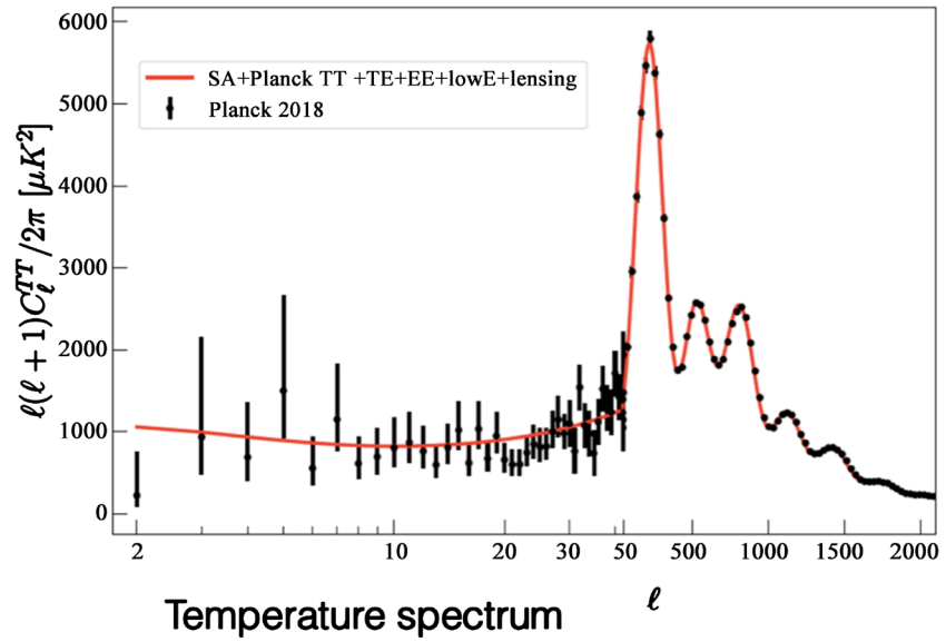
Figure 2. Corrected CMBR data points included in this plot.
