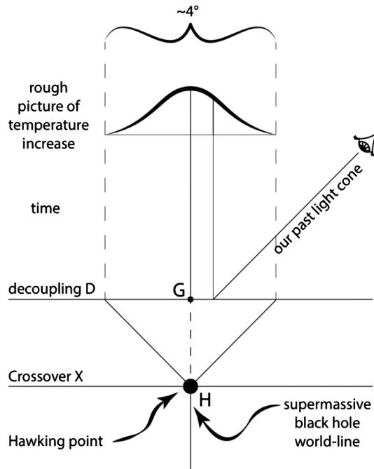
Figure 1. As given in [4] which has competing black hole radiation, and can we see this today in the CMBR?
