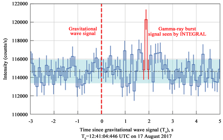
Figure 3. from [13] states that there would be close synchronization of time between a gravitational wave signal, and gamma ray bursts, in an event likely connected to a quark star being formed.
