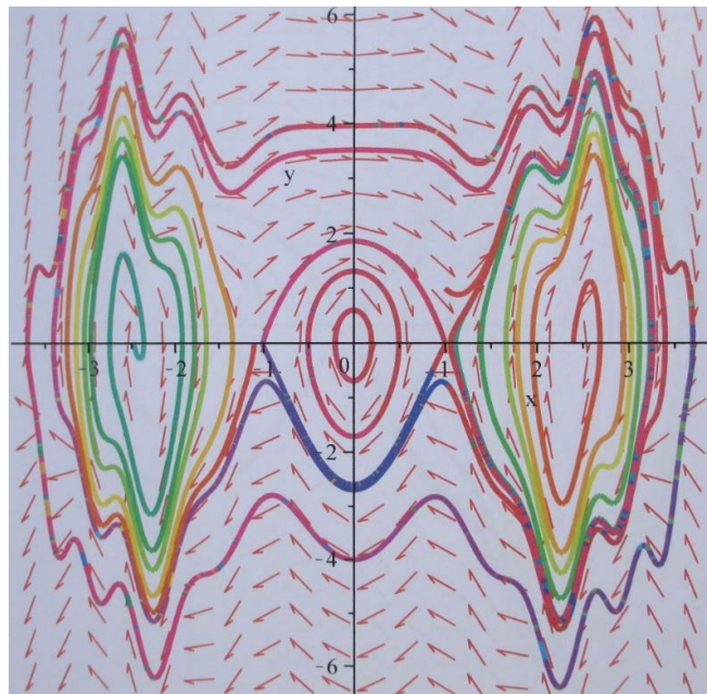
Figure 6. One stable center with stable closed curves.
