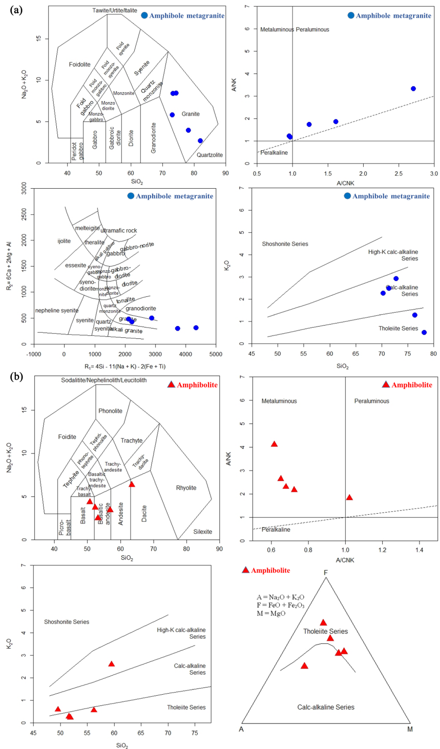
Figure 9. Classification diagrams of the different formations of the Alépé area. (a) Amphibole metagranite) and (b) Amphibolite): diagram Na 2 O + K 2 O according to SiO 2 of Middlemost (1994) of plutonites and volcanites. (a) Amphibole metagranite) and (b: Amphibolite): classification using R 1 and R 2 parameters (after De la Roche et al. , 1980), calculated on the basis of the proportions of elements in millication. (a) Amphibole metagranite) and (b: Amphibolite): A/NK vs A/CNK diagram after Shand (1934). (a) Amphibole metagranite): K 2 O vs. SiO 2 diagram from Peccerillo and Taylor (1976); (b) Amphibolite): AFM diagram of Irvine and Baragar (1971).
