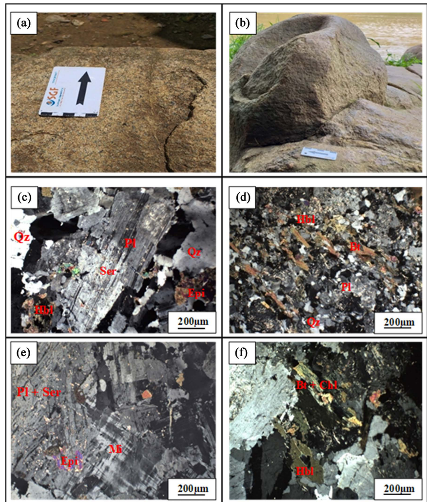
Figure 5. Macroscopic and microscopic aspects of amphibole metagranite. (a) and (b): Macroscopic aspect; (c)-(f): Microscopic aspect. Qz: quartz. Pl: plagioclase. Bt: biotite. Hbl: hornblende. Ser: sericite. Epi: epidote. Chl: chlorite. Op: opaque.
