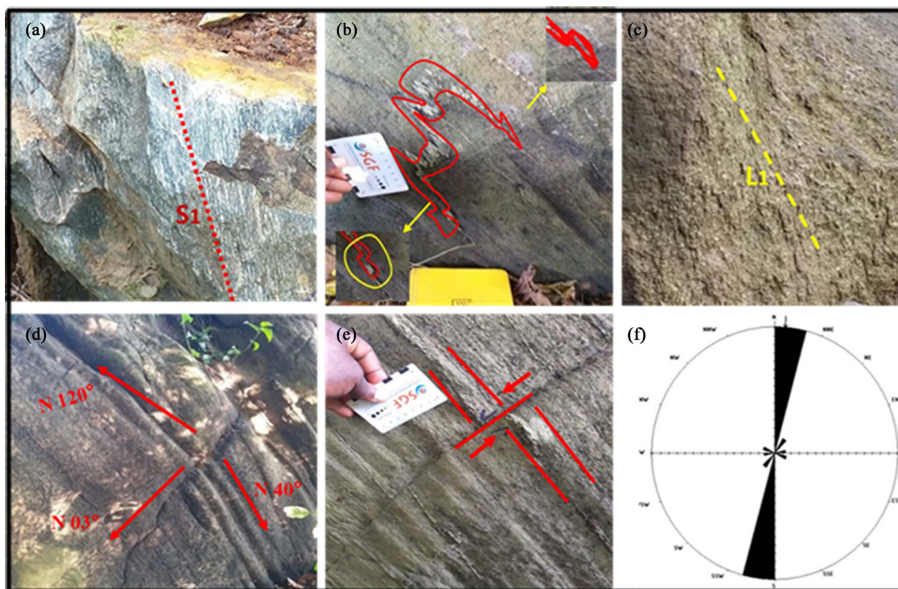
Figure 7. (a) Foliation in the amphibolite. (b) M-hinged, Z- and S-flanked entrainment fold marking dextral shear. (c) Subvertical mineral stretching lineation observed in the amphibole metagranite. (d) Fracture set. (e) Sinister break-up. (f) Directional rosette of the veins.
