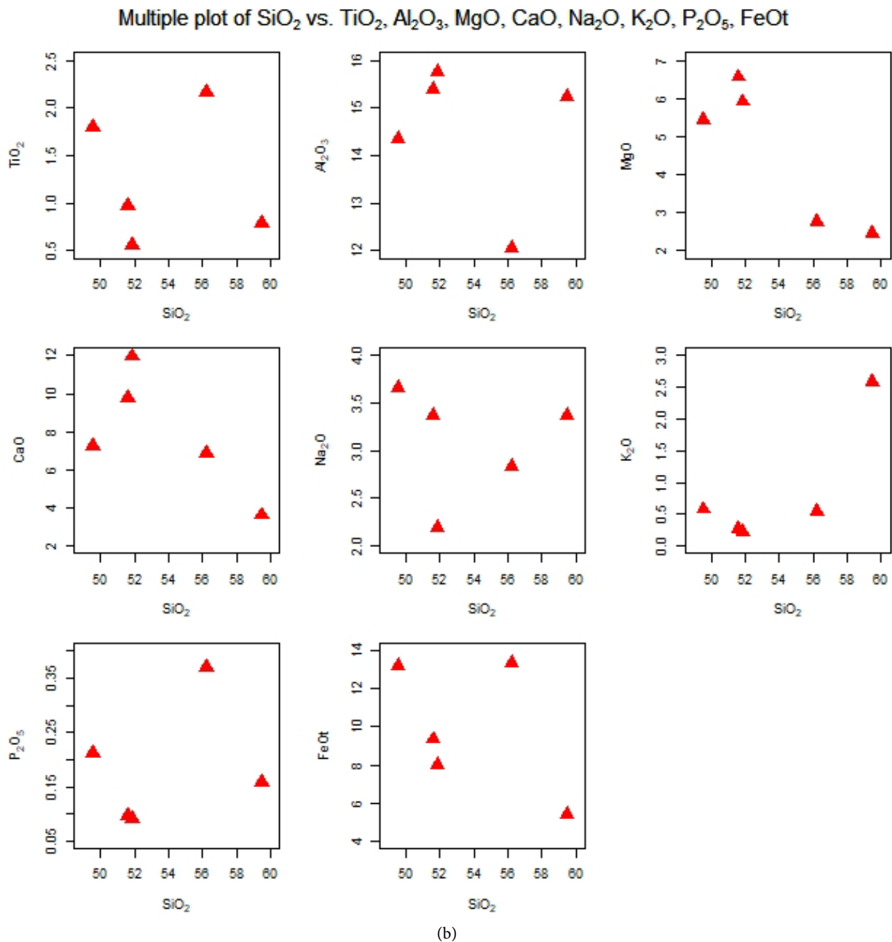
Figure 10. (a) Amphibole metagranite) and (b) Amphibolite) distribution of the formations in the study area (Alépé) in the Oxides vs \text{SiO}_2 Harker diagrams.
