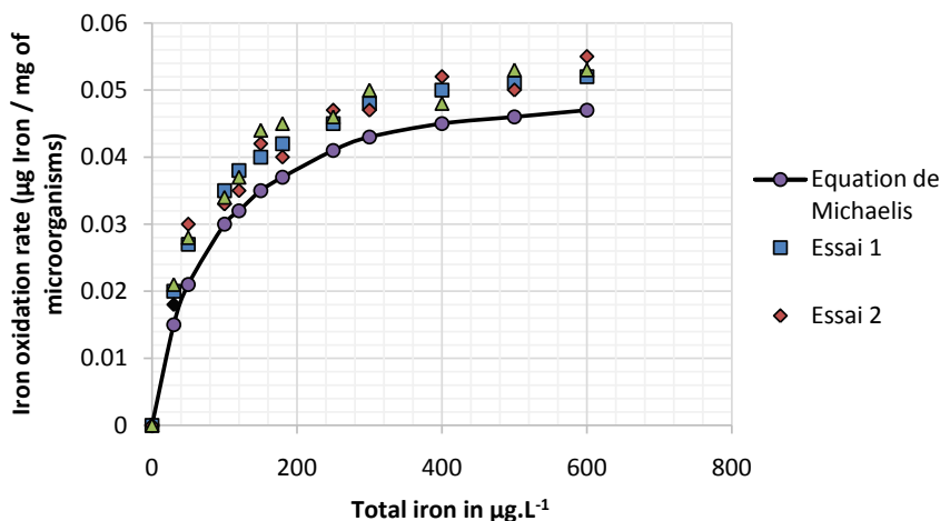
Figure 8. Fe (II) oxidation rate versus Fe (II) concentration, showing the Michaelis-Merten oxidation kinetics for Fe (II) at T = 25^{\circ}\text{C} \pm 1^{\circ}\text{C} , \text{pH} = 9.5 and [\text{O}_2] = 6.5 \text{ mg}\cdot\text{L}^{-1} .
