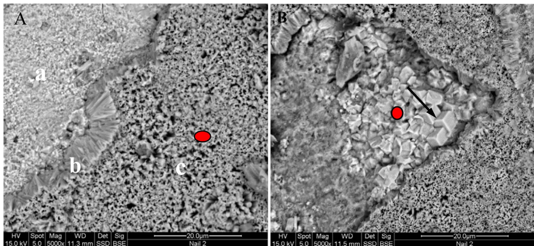
Figure 24. (A) Goethite (a), scaly sheaf-like lepidocrocite (b) and coraline-like akaganeite (c) (Table 5, An. 25). (B) Magnetite crystallites substratum (a) beneath a fine (~10 \mu\text{m} thick) fibrous crust of akaganeite. The presence of Cl is contamination from neighboring akaganeite. We attribute the moderate C concentration to traces of organic carbon remaining from the original bacterial source. Chemical analysis (Table 5, An. 26 red marker) is on magnetite beneath a veneer of akaganeite. The dominant crystal forms (at arrow) appear to be cubic and/or cuboid (rectangular shaped).
