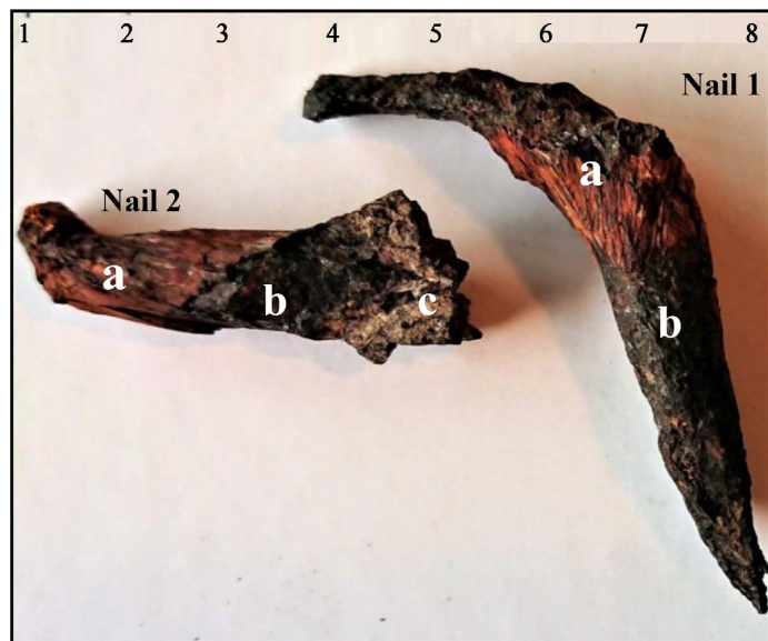
Figure 21. Two iron nails extricated from their source. Key: a-petrified wood, b- oxidized iron covering a metallic iron core, c-carbonate flowstone veneer with calcite, aragonite, gypsum and ankerite (Table 6, An. AS 6). The head area of Nail 1 (left edge) and bottom of Nail 2 (left edge) are both bent and the extremities are broken off. Indents in the nails made by hammering are not clearly visible in the photos.
