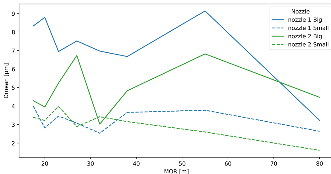
Figure 8. Dmean for nozzle 1 (selected nozzle) and nozzle 2 (currently used nozzle) for different MOR ranges. For both nozzles, the 2 fog configurations, that of the biggest droplets and that of the smaller droplets, are shown.
