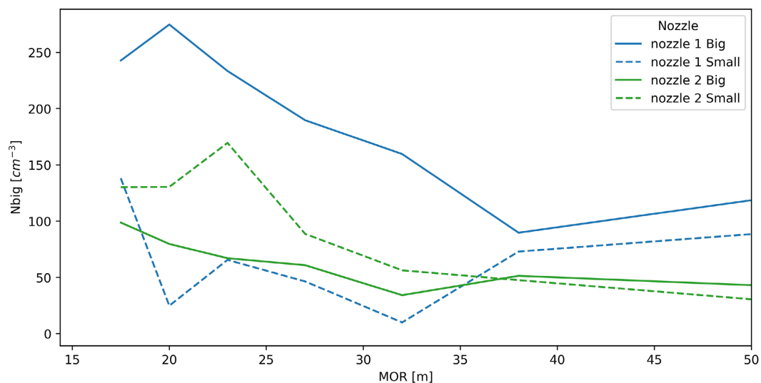
Figure 9. The number of big droplets, Nbig, for nozzle 1 (selected nozzle) and nozzle 2 (currently used nozzle) for different MOR ranges inferior to 50m. For both nozzles, the 2 fog configurations, that of the biggest droplets and that of the smaller droplets, are shown.
