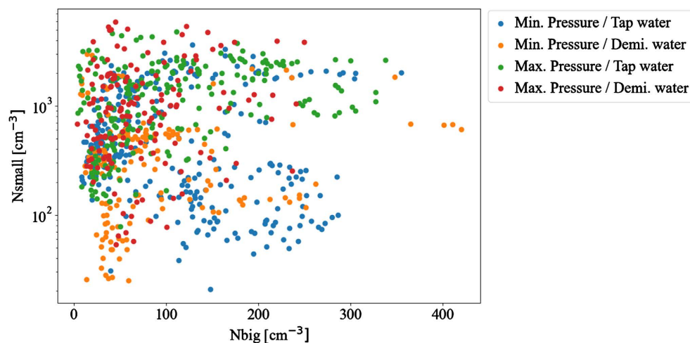
Figure 3. Nbig depending on Nsmall for all the nozzles with different combination of water and pressure.
