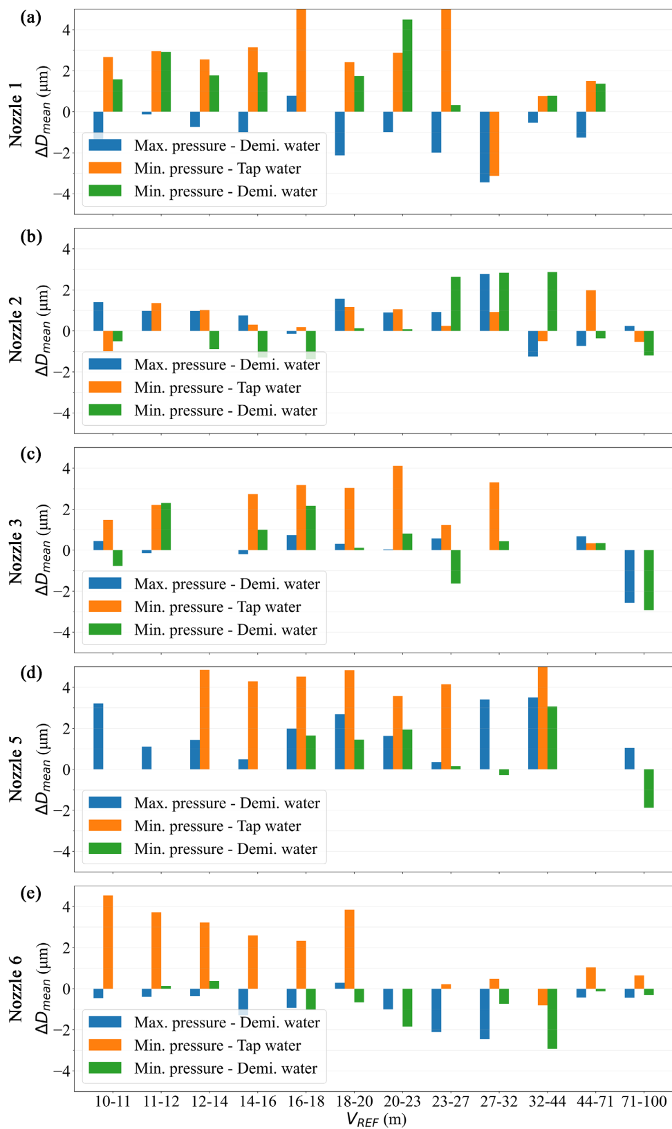
Figure 5. Dmean discrepancy compared to the reference (Maximum pressure and Tap water) for all the significant nozzles (a) represents the nozzle 1, (b) the nozzle 2, (c) the nozzle 3, (d) the nozzle 5 and (e) the nozzle 6.
