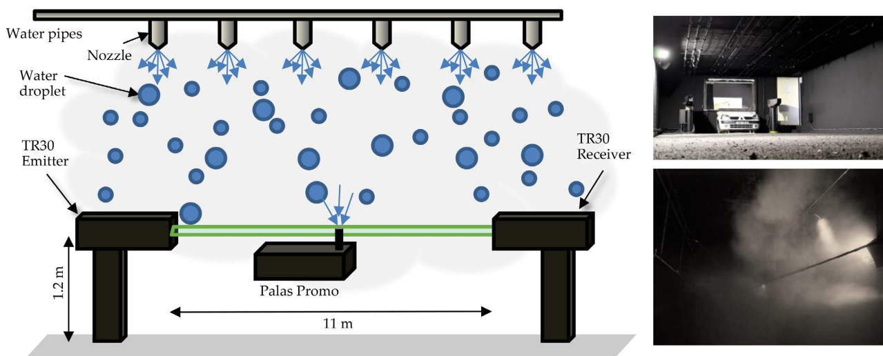
Figure 1. Schema of the experiment, and pictures of the facility.
