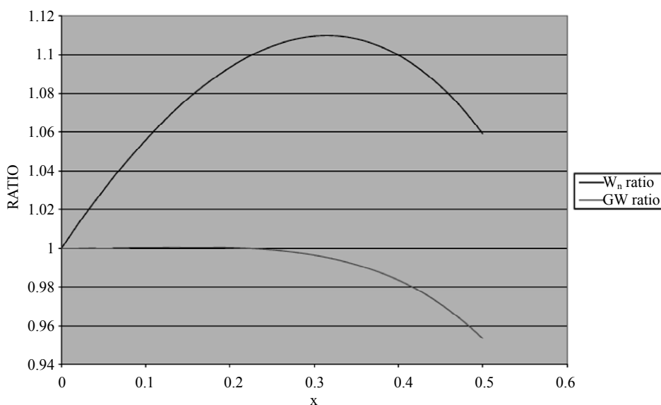
Figure 2. Relative welfare, \gamma = \frac{10}{11} .
