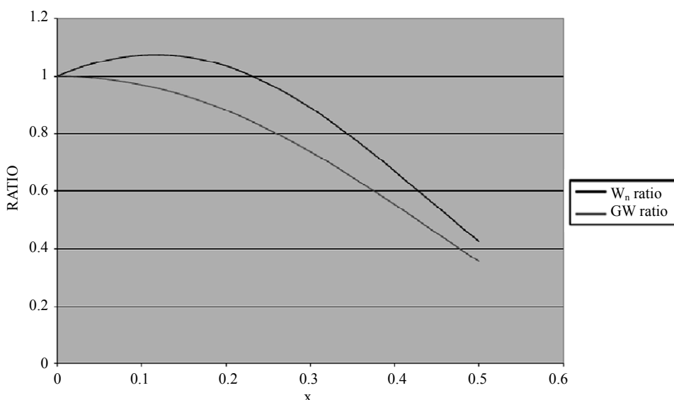
Figure 1. Relative welfare, \gamma = 5 .
