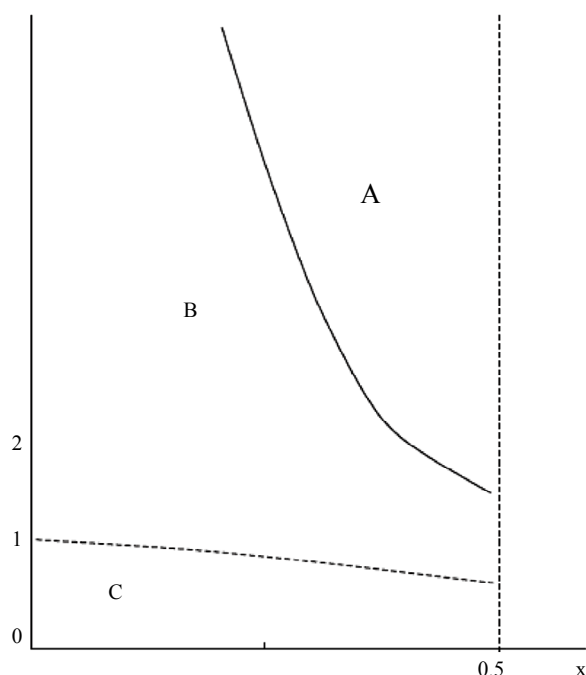
Figure 3. The relation between elasticity of innovation, \gamma and x .
