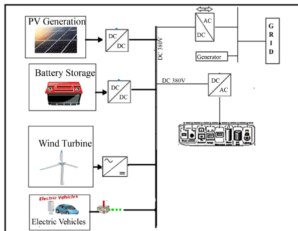
Figure 3. A residential micro-grids and with energy storage [4].
