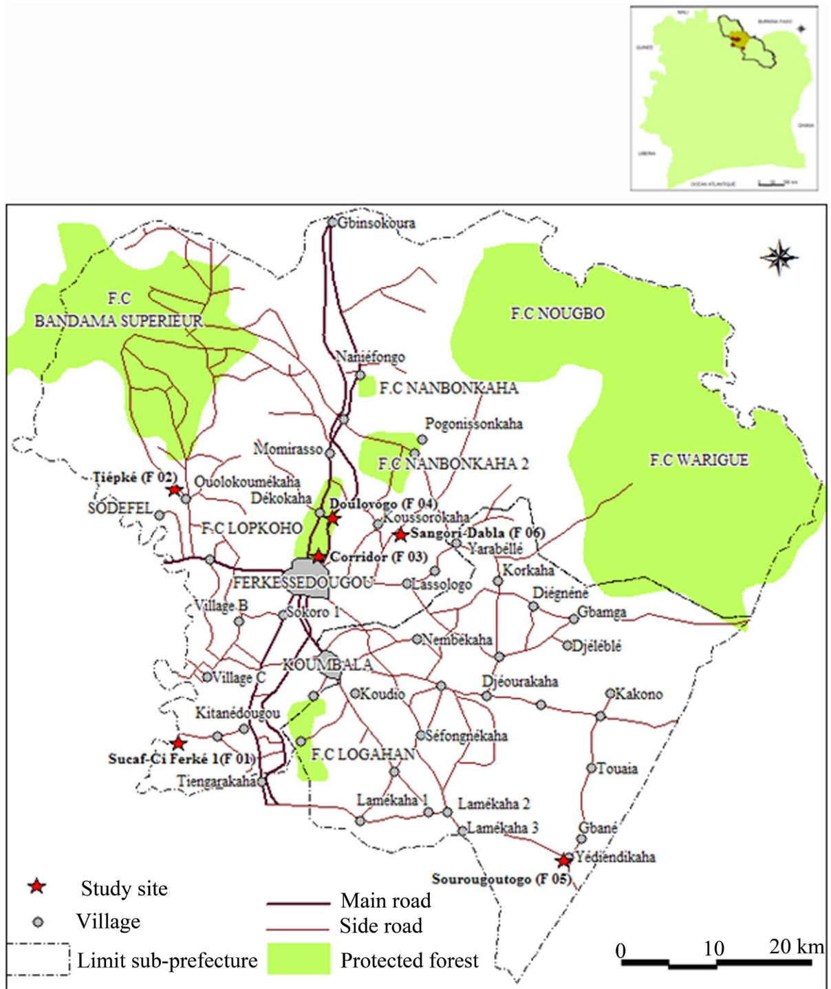
Figure 1. Study locations.
