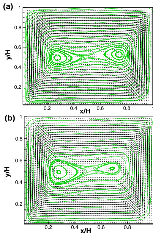
Figure 4. Velocity vectors and stream lines for (a) pure fluid ( H_2O ) and (b) nanofluid ( H_2O-Cu ).
