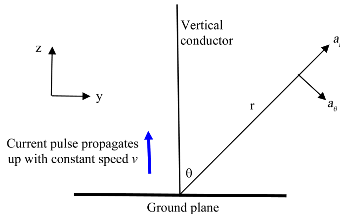
Figure 1. The geometry relevant to the derivation of field equations pertinent to the transmission line model. Note that a_r and a_\theta are unit vectors in the direction of increasing r and \theta .
