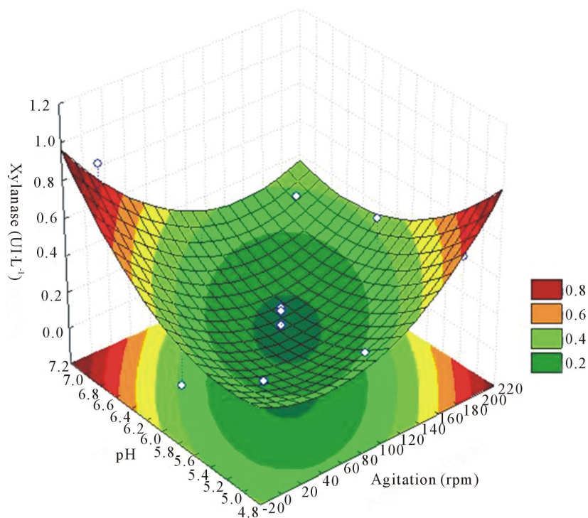
Figure 2. Response surface for purposes of agitation and different pH on the xylanase production at 12 days of cultivation on L. edodes .
