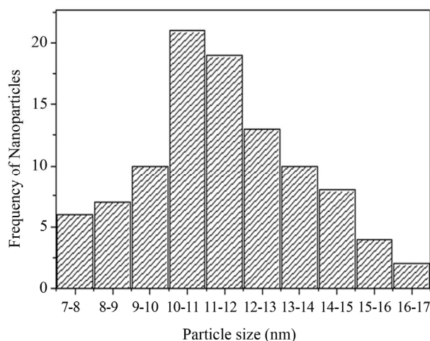
Figure 3. Histogram of frequency of particles versus their particle size.
