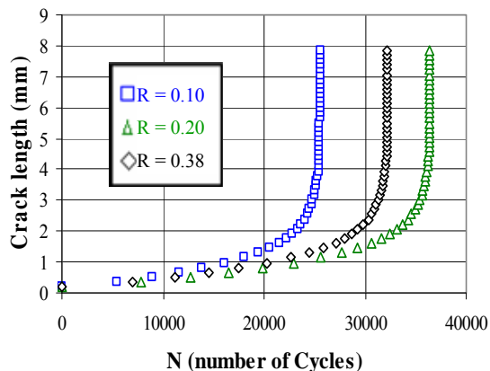
Figure 2. Effect of stress ratio on fatigue life for X60 pipeline material.
