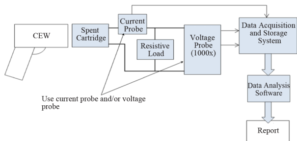
Figure 5. Schematic diagram of CEW test setup.
