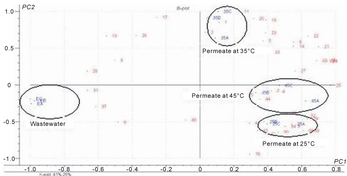
Figure 2. Scores and loading plots for PC1 × PC2. Numbers in the loading plots represent the peak number showed in Table 1.
