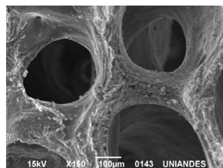
Figure 2. SEM microphotograph. Partial view of carbonized CHUOX surface. Magnification: × 150.
