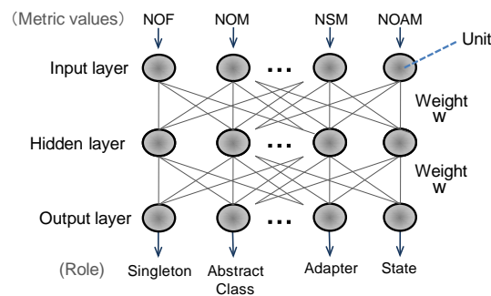
Figure 8. Overview of the neural network.
