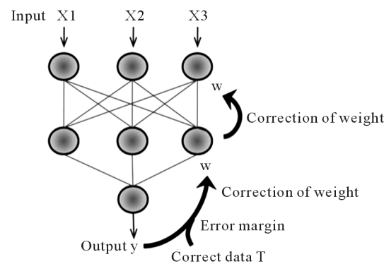
Figure 9. Back propagation.
