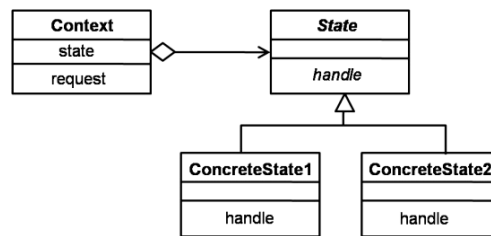
Figure 1. State pattern.
