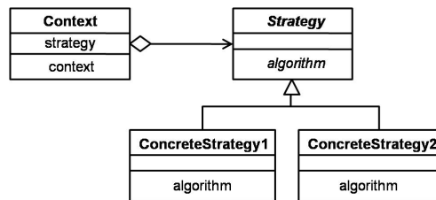
Figure 2. Strategy pattern.
