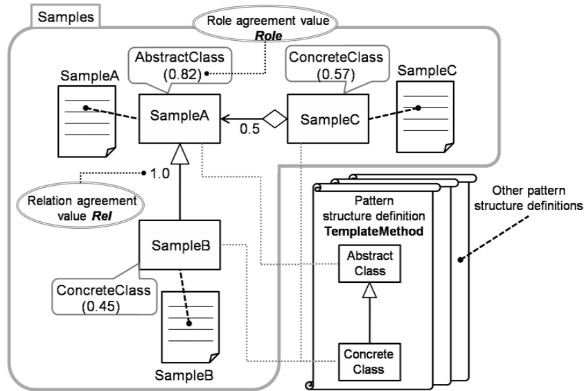
Figure 11. Example of detecting Template Method pattern.
