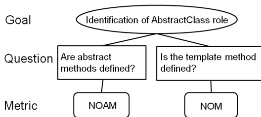
Figure 6. Example of GQM application result (AbstractClass role).
