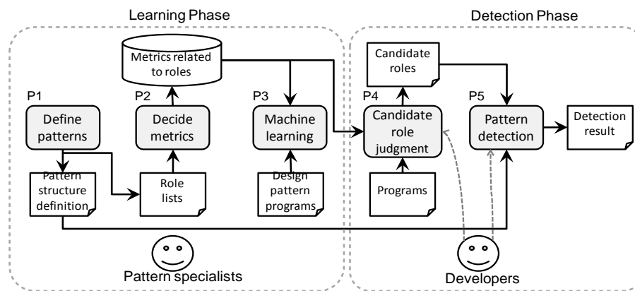
Figure 5. Process of our technique.
