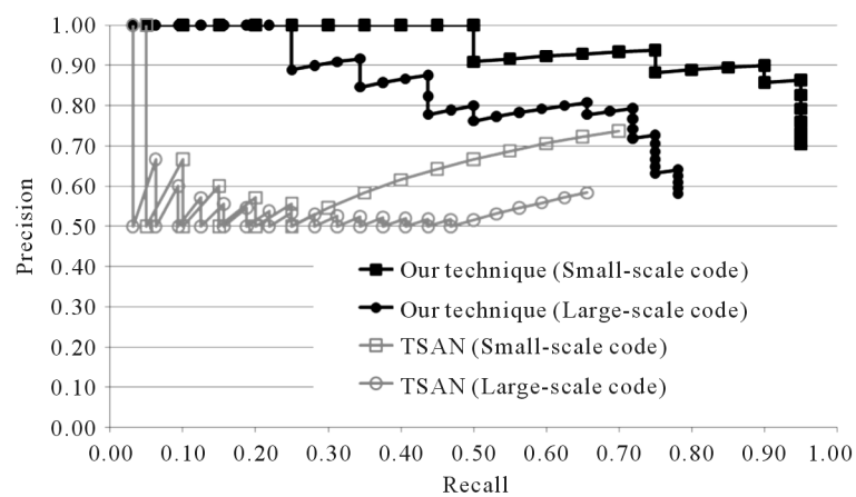
Figure 12. Recall-precision graph (vs. TSAN).
