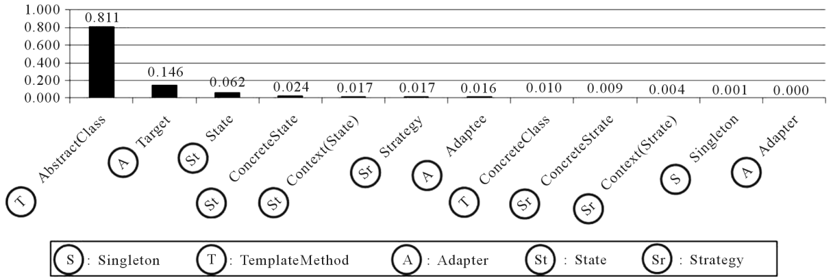
Figure 10. Example of machine learning output.
