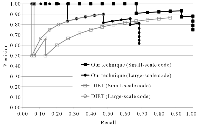
Figure 13. Recall-precision graph (vs. DIET).
