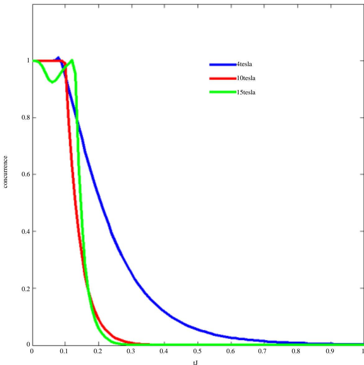
Figure 5. (Color online) The time ( tJ ) evolution of entanglement for the initial two-qubit state
