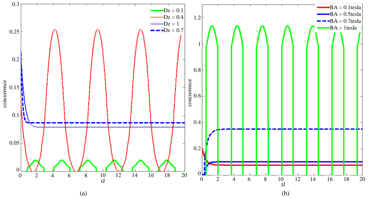
Figure 6. (Color online) The time ( tJ ) evolution of entanglement for the initial two-qubit entangled state |\Phi\rangle = (1/\sqrt{2})(\cos\vartheta|01\rangle + \sin\vartheta|10\rangle) ; (a) for different values of D_z , setting: B_z = B_A = 0 tesla, (b) for different values of the anisotropy field B_A , setting D_z = 1 , other parameters are set to J_z = 1 = \Omega = 1 , B_z = 1 tesla, \vartheta = \pi/4 .
