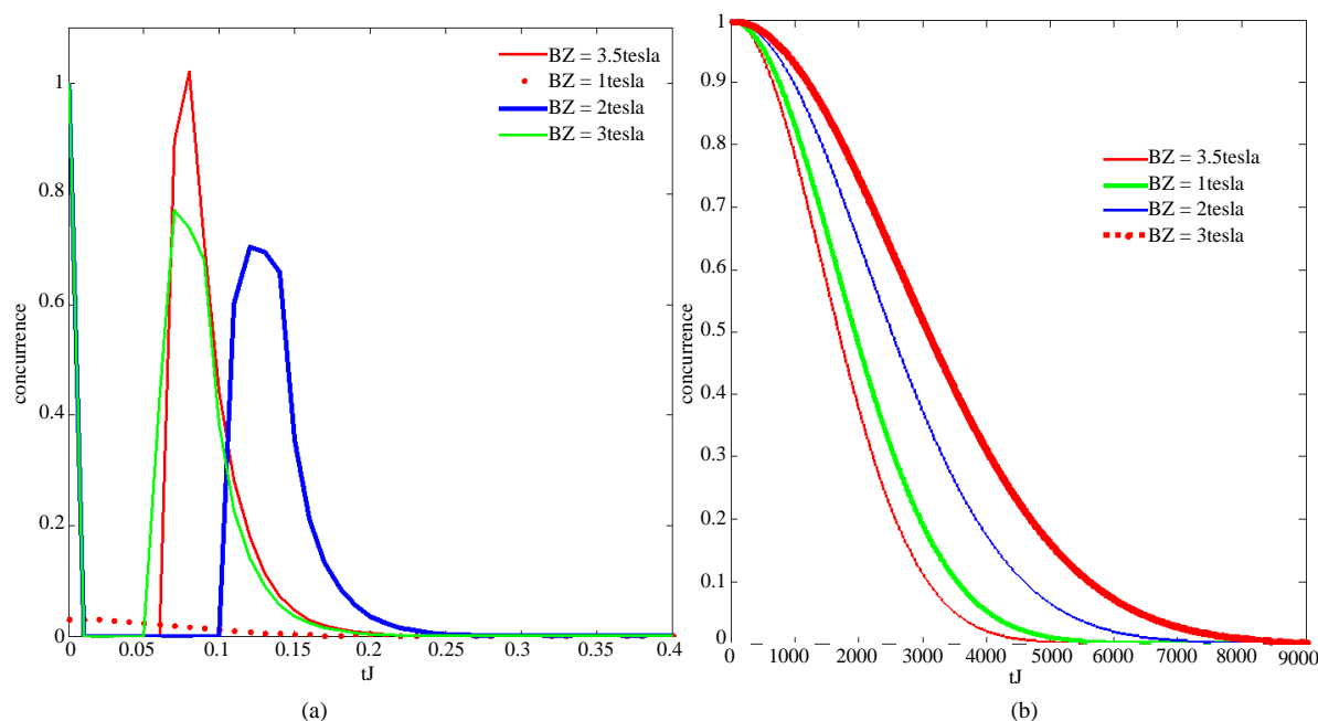
Figure 2. (Color online) The time ( tJ ) evolution of entanglement for the initial two-qubit state |\Phi\rangle = (1/\sqrt{2})(\cos\mathcal{G}|00\rangle + \sin\mathcal{G}|11\rangle) for different global static external magnetic field (a) finite size of the AF spin environment N = 100 ; bg = J_o/\sqrt{N}g\mu_B = 1 tesla is induced magnetic field due to system-environment coupling (b) thermodynamic limit, others parameters are set to J_z = 1 , B_A = 1 tesla, MSJ/g\mu_B = 100 tesla, \mathcal{G} = \pi/4 , T/g\mu_B = 3.5 tesla.
