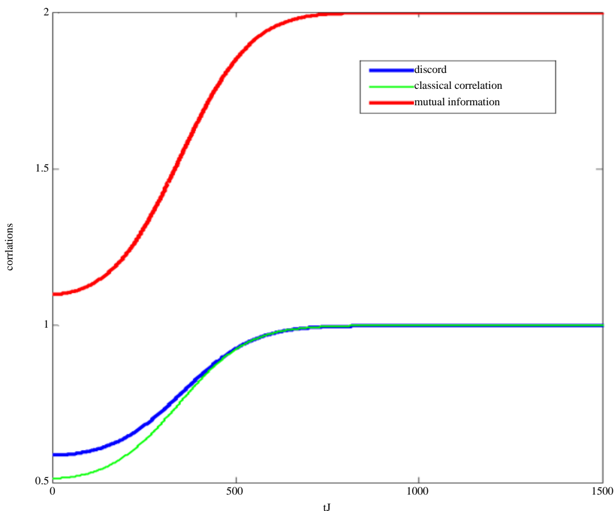
Figure 8. (Color online) The time ( tJ ) evolution of quantum correlations in the thermodynamic limit : discord (blue curve), classical correlation (green curve), mutual information (red curve) for the initial two-qubit state |\Phi\rangle = (\cos\vartheta|00\rangle + \sin\vartheta|11\rangle) ; system parameters are set to J_z = 1 , B_A = 0.1 tesla , MSJ/g\mu_B = 100 tesla , T/g\mu_B = 3.5 tesla , B_z = 2 tesla , \vartheta = \pi/4 , l = 1/8 , k = 7/8 .
