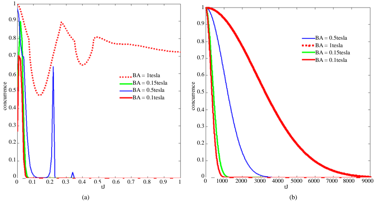
Figure 3. (Color online) The time ( tJ ) evolution of entanglement for the initial two-qubits state |\Phi\rangle = (1/\sqrt{2})(\cos\vartheta|00\rangle + \sin\vartheta|11\rangle) for different anisotropy field; (a) finite size of the AF spin environment N = 100 ; bg = 1 tesla, MSJ/g\mu_B = 1 tesla; (b) thermodynamic limit, MSJ/g\mu_B = 100 tesla, others parameters are set to J_z = 1 , B_z = 0.5 tesla, T/g\mu_B = 3.5 tesla, \vartheta = \pi/4 .
