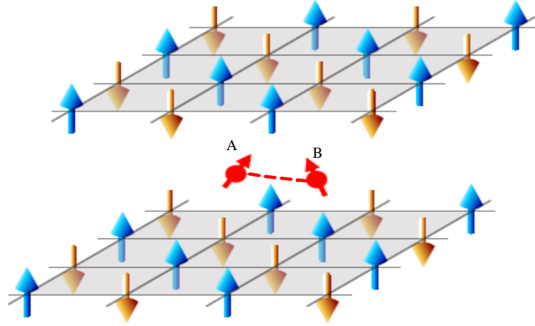
Figure 1. (Color online) Schematic of the two-qubit systems interacting with common anti-ferromagnetic environment.
