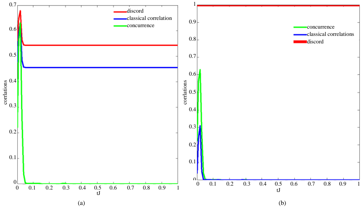
Figure 7. (Color online) The time ( tJ ) evolution of various correlation for the initial two-qubit entangled state |\Phi\rangle = (\cos\vartheta|00\rangle + \sin\vartheta|11\rangle) ; (a) for minimization parameters l = 1/8 , k = 7/8 ; (b) for minimization parameters l = k = 1/2 , others parameters are set to J_z = 1 , B_A = 0.1 tesla, bg = 1 tesla, MSJ/g\mu_B = 1 tesla, T/g\mu_B = 3.5 tesla, B_z = 2 tesla, \vartheta = \pi/4 .
