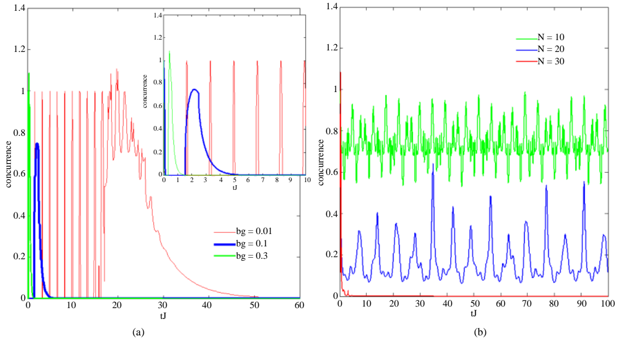
Figure 4. (Color online) The time ( tJ ) evolution of entanglement for the initial two-qubit state |\Phi\rangle = (1/\sqrt{2})(\cos\vartheta|00\rangle + \sin\vartheta|11\rangle) ; (a) for different induced field bg = J_o/\sqrt{N}g\mu_B for N = 100 , (b) different sizes of the AF spin environment N for bg = 1 tesla; N = 10 (green curve), N = 20 (blue curve), N = 30 (red curve), others parameters are set to J_z = 1 , B_A = 0.15 tesla, MSJ/g\mu_B = 100 tesla, T/g\mu_B = 1.7 tesla, B_z = 1 tesla, \vartheta = \pi/4 .
