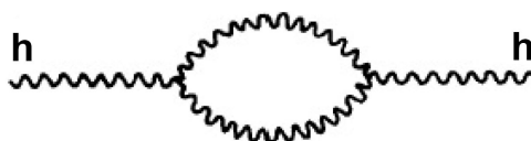
Figure 4. The one-loop graviton self-energy diagram.
