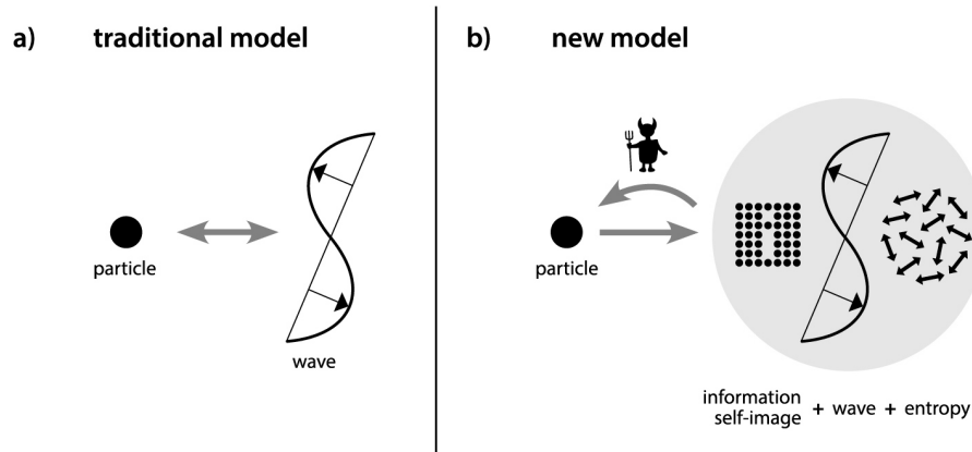
Figure 1. The particle-wave duality in conventional quantum physics (a) and within the dynamic energy model (b) in which information on matter is involved in the backformation of the particle from the wave.
