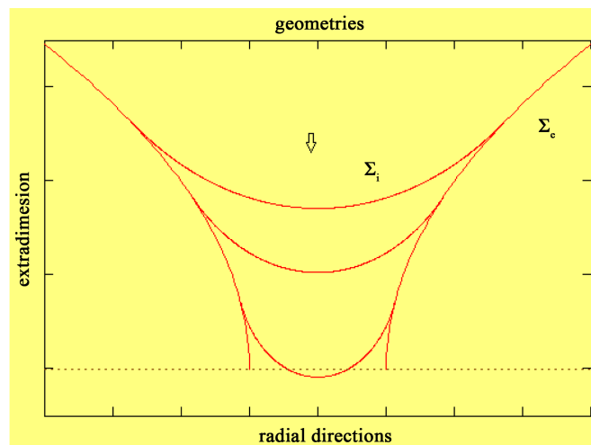
Figure 1. The inner surface and the outer surface of the whole Schwarzschild model.
