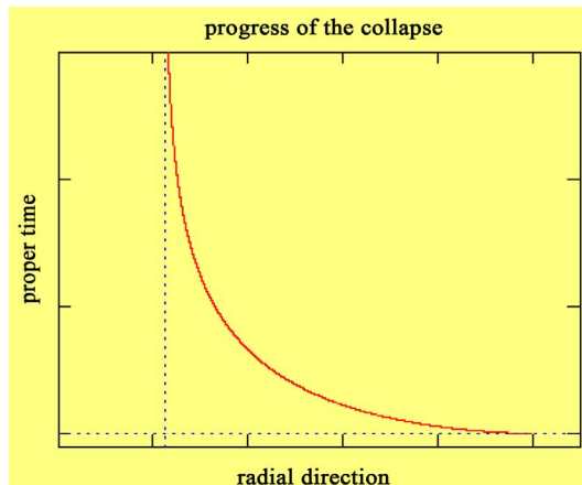
Figure 2. The star needs an infinitely long time to reach the minimum radius.
