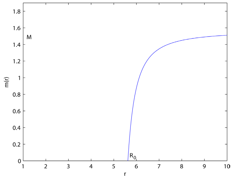
Figure 2. The graph of m(r) .
