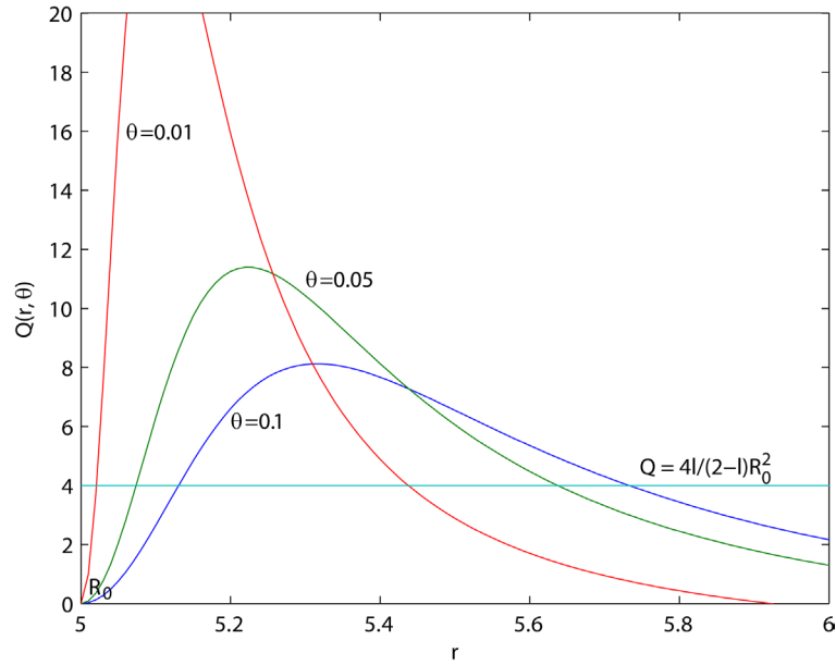
Figure 3. Plot showing that if \theta \rightarrow 0 , then r_1 \rightarrow R_0 .
