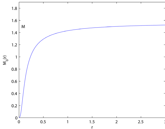
Figure 1. The graph of the smeared mass M_\theta(r) .
