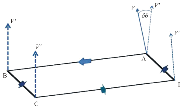
Figure 1. Parallel transport: The vector V is parallel transported in a closed circuit. Upon arrival at its original position, the vector is not equal to the original vector and this is a result of the curvature of the space in question.
