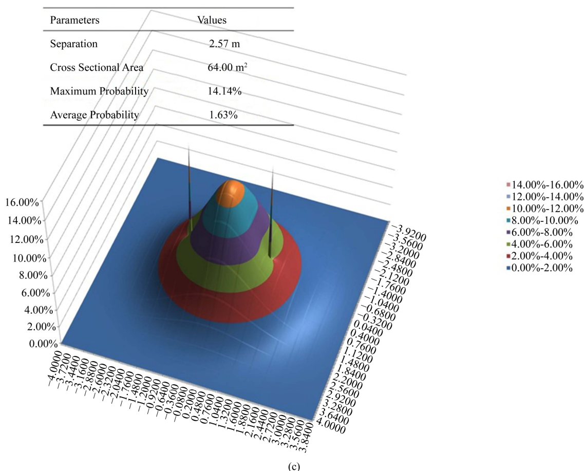
Figure 5. (a) Joint probability at 0.1 m separation; (b) Joint probability at 0.4 m separation; (c) Joint probability at 2.6 m separation.
