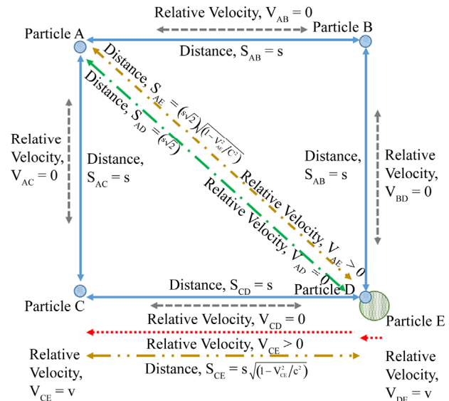
Figure 1. The 5-particle box paradox.
