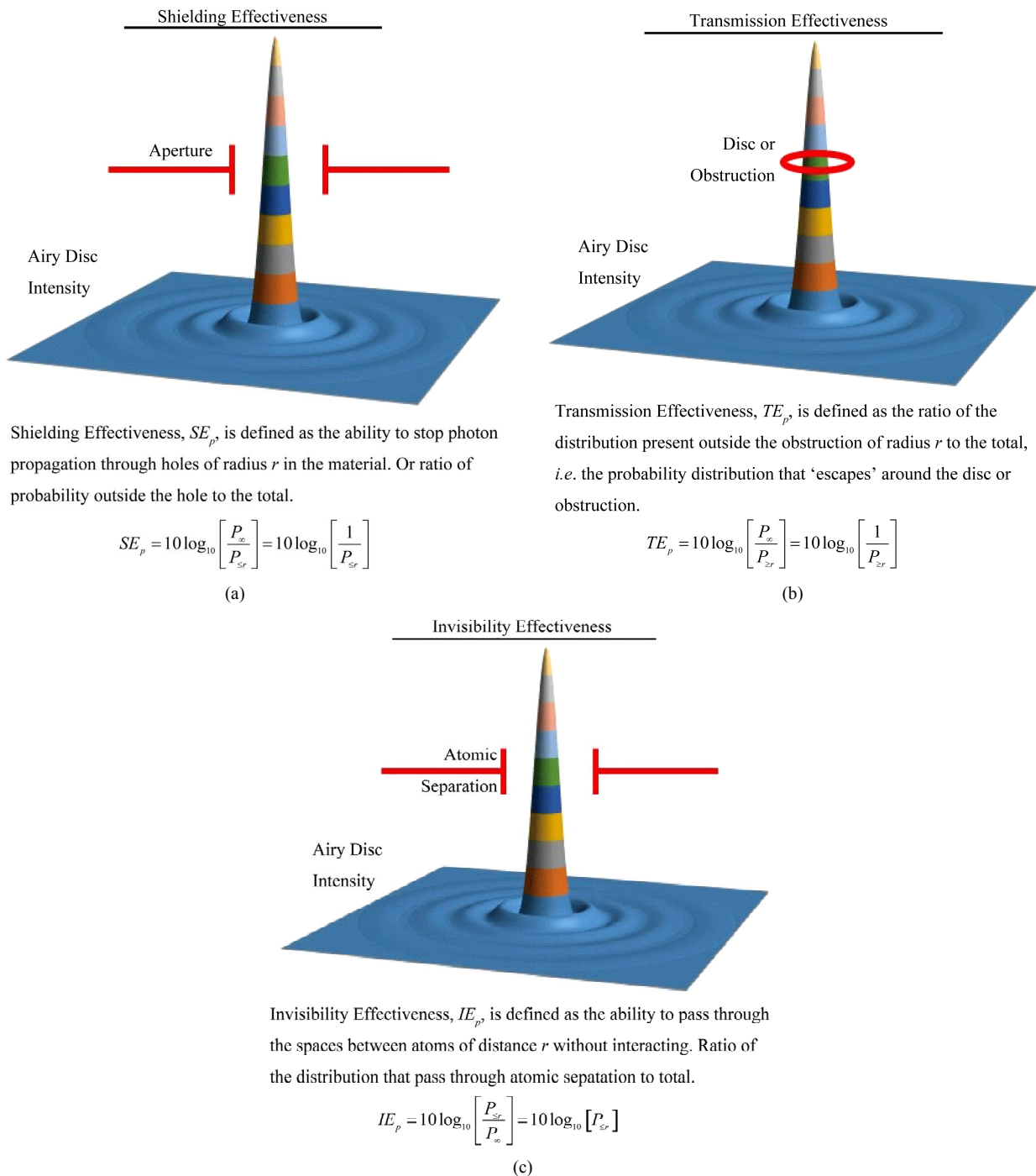
Figure 2. (a) Photon shielding; (b) Photon transmission; (c) Photon invisibility.
