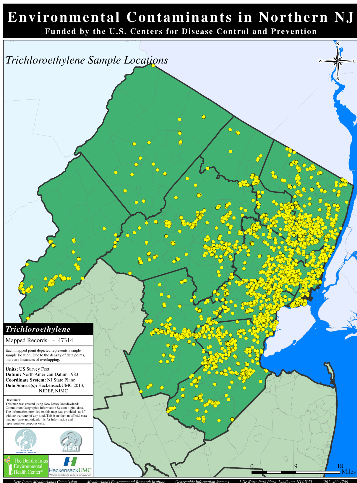
Figure 6. Trichloroethylene sample locations.
