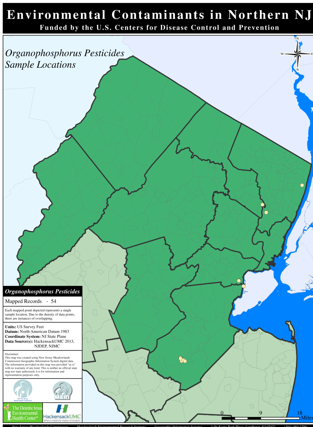
Figure 8. Organophosphorus pesticides sample locations.
