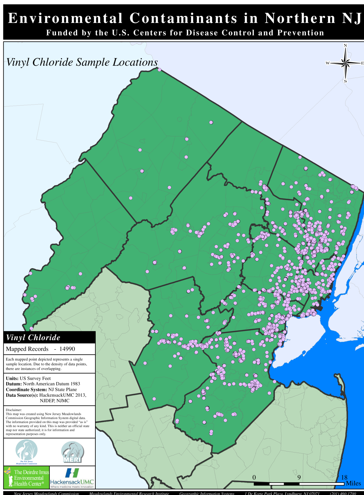
Figure 7. Vinyl Chloride sample locations.
