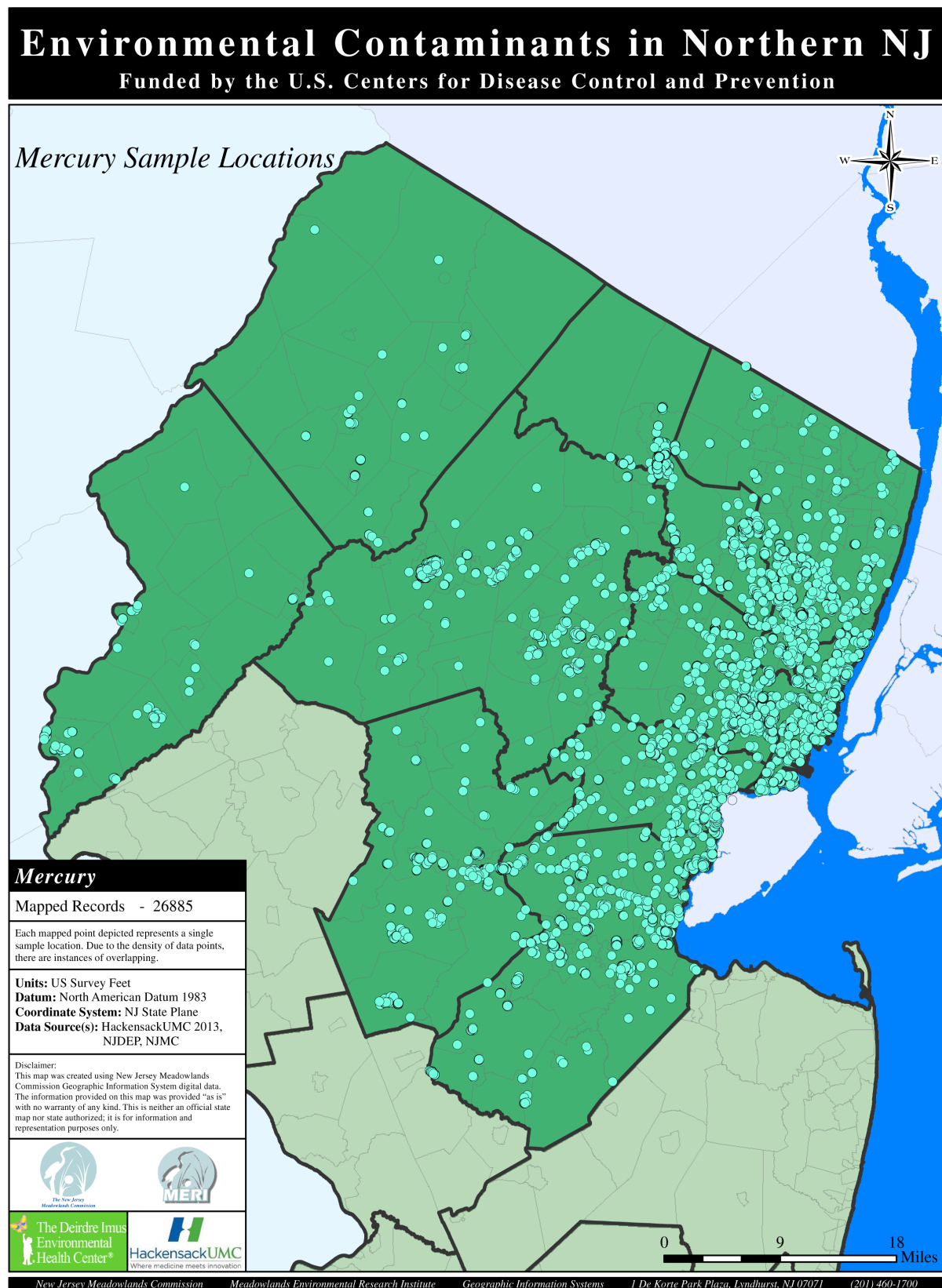
Figure 4. Mercury sample locations.
