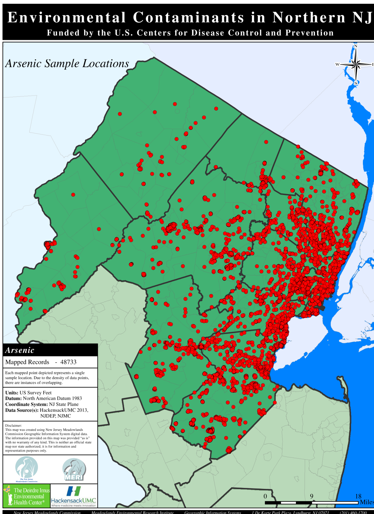
Figure 1. Arsenic sample locations.
