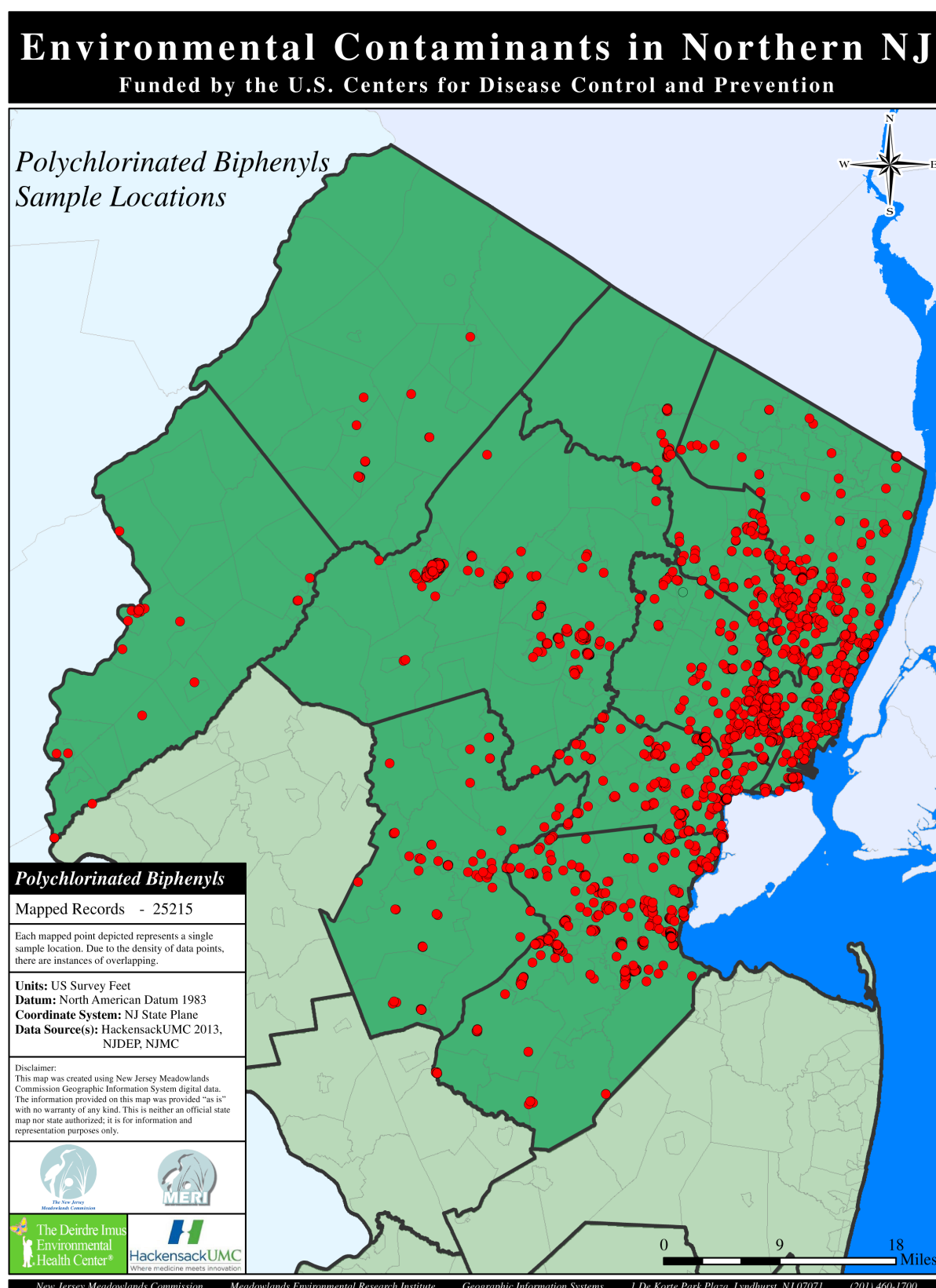
Figure 5. Polychlorinated biphenyls sample locations.
