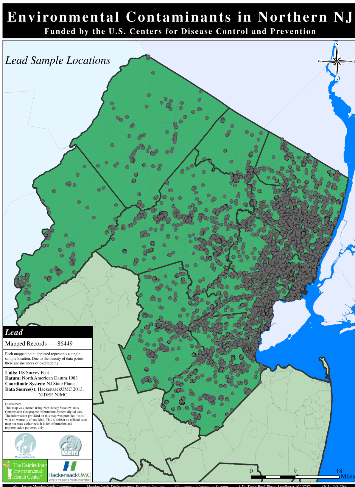
Figure 2. Lead sample locations.
