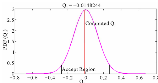
Figure 3. Graphical validation process Krige Method using the software tool “EasyKrig”.
