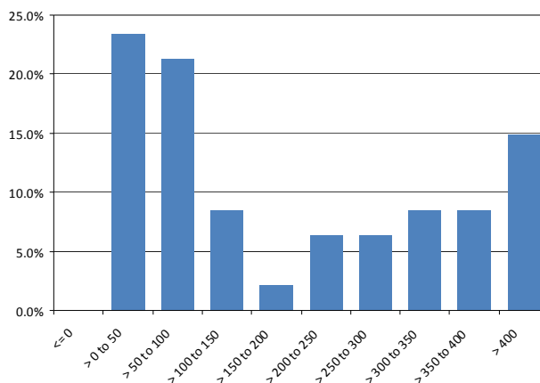
Figure 8. Summary of building lengths (ft) (n = 47).
