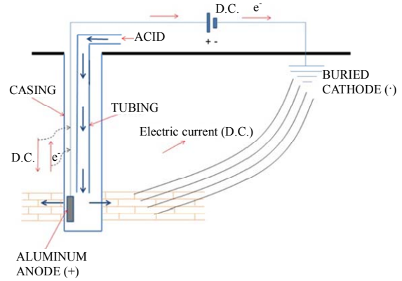
Figure 2. Electrodes arrangement for acidizing operation.
