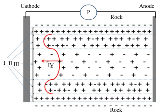
Figure 1. Schematic diagram of electrokinetic double layer (I: Immobile Double Layer, II: Mobile Double Layer, III: Free Water, IV: Velocity Profile) as envisioned by the authors. Solid curved line—velocity profile in a capillary. P = D.C. current power supply. Rock is negatively charged [8].
