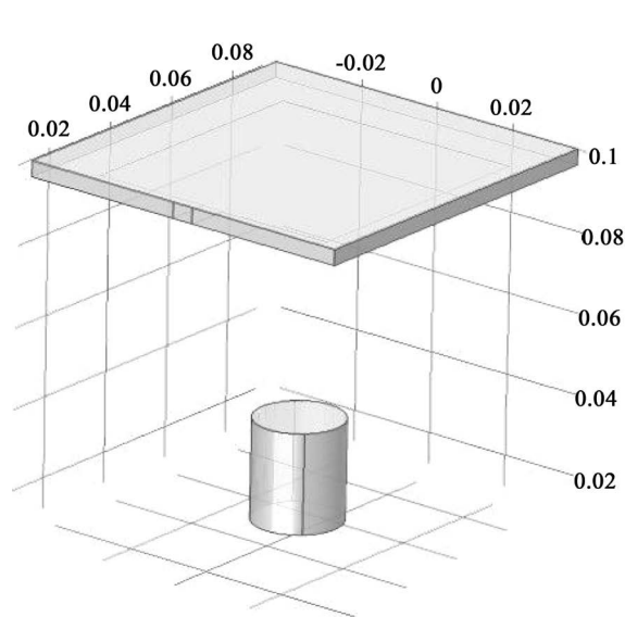
Figure 1. The model using in COMSOL for simulating. This Image shows the antenna used to generate the EM wave (Top) and the brain tissue sample (Bottom).
