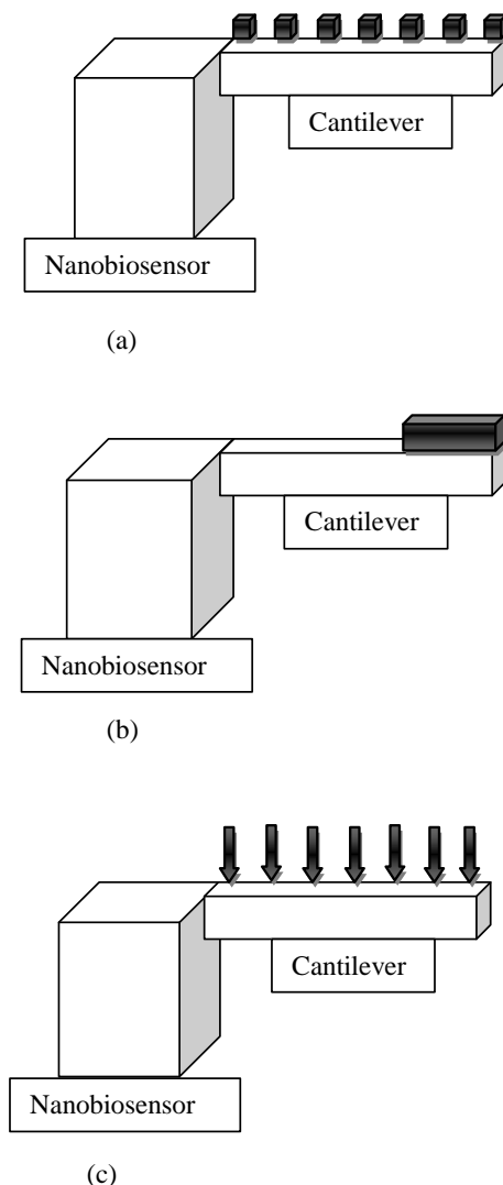
Figure 3. (a) Cantilever experiencing surface stress; (b) Cantilever experiencing mass load; (c) Cantilever experiencing temperature change.
