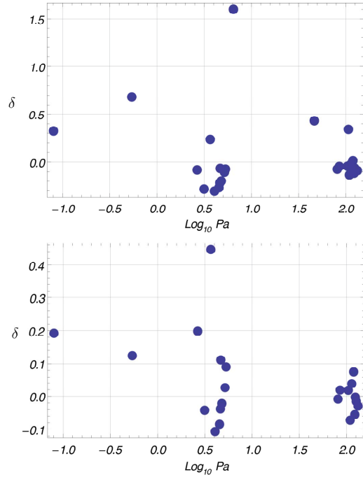
Figure 2. Plots of \delta = (r'_{ij} - r_{ij}) / x_{ij} versus x_{ij} (observed \log_{10} amplitude) for scenario 1 (top) and scenario 2 (bottom). Positive values indicate that the BOOM model provides a better fit to the calibration explosions.
