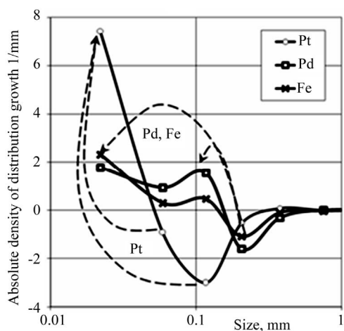
Figure 1. Grain-size class redistribution of platinum, palladium and iron after a storage period of 4 years.
