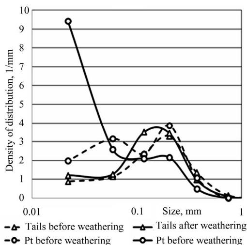
Figure 2. Grain-size class redistribution of tails material and platinum.
