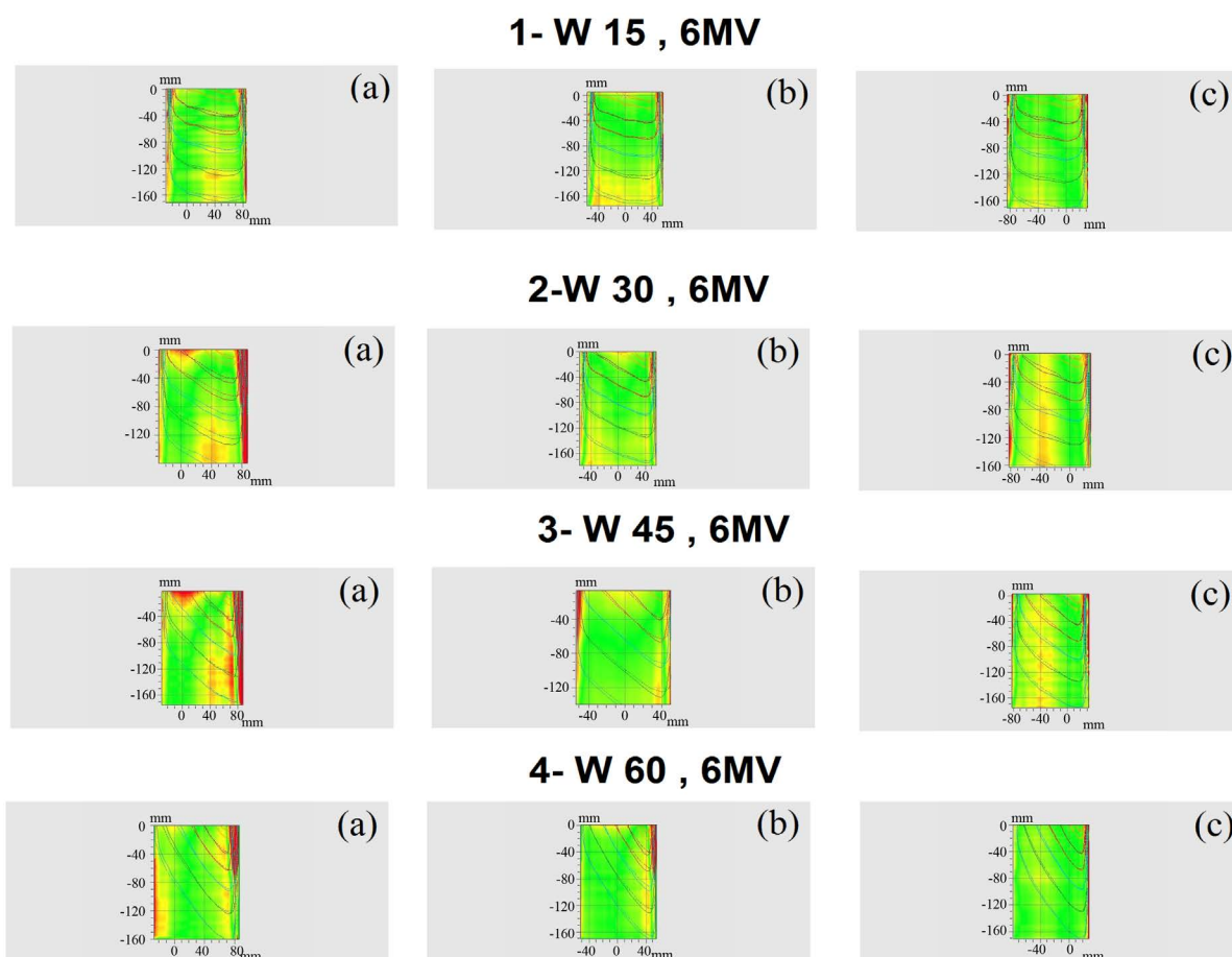
Figure 2. Gamma distribution for different field using the superposition algorithm for 15, 30, 45 degrees and 60 degrees physical wedge (PW), for 6 MV. The upper parts of the distributions represent the low-dose region of the wedged field; green indicates regions where \gamma \leq 1 ; and red indicates \gamma > 1 (individual criteria: \Delta\%D = 3\% , DTA = 3 mm).
