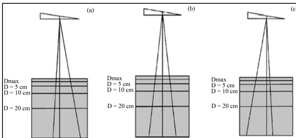
Figure 1. View of the beam setup showing the depths of measurement (a) in the asymmetrical setting ( X1 = 5 , X2 = 5 , Y1 = 2.5 , Y2 = 7.5 ), (b) in the symmetrical setting ( X1 = 5 , X2 = 5 , Y1 = 5 , Y2 = 5 ), and (c) in the asymmetrical setting ( X1 = 5 , X2 = 5 , Y1 = 7.5 , Y2 = 2.5 ).
