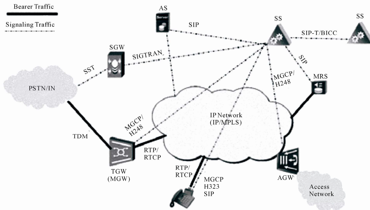
SGW = Signaling Gateway, AS = Application Server, SS = Softswitch, MRS = Media Resource Server, TGW = Trunking Gateway, AGW = Access Gateway
