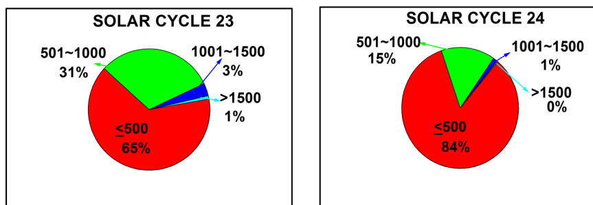
Figure 1. Shows the distribution of total CMEs according to CME's speed for ascending phase of solar cycles 23 and 24.
