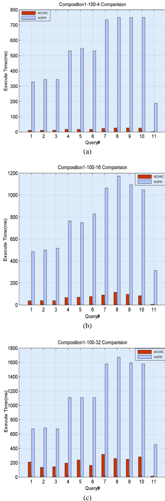
Figure 10. Efficiency compare in Composition1-100 set. (a) Efficiency compare in 100-4 set; (b) Efficiency compare in 100-16 set; (c) Efficiency compare in 100-32 set.
