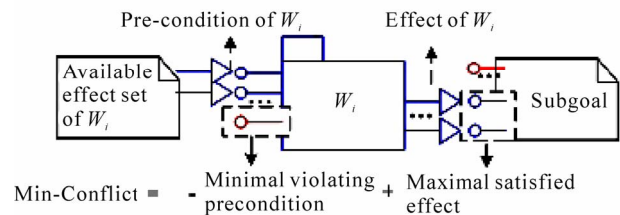
Figure 5. The definition of min-conflict.
