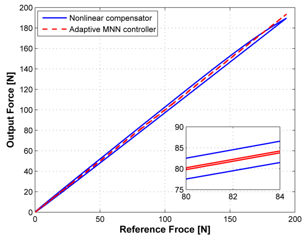
Figure 9. Comparison of the force hysteresis loop between nonlinear compensator and adaptive controller.
