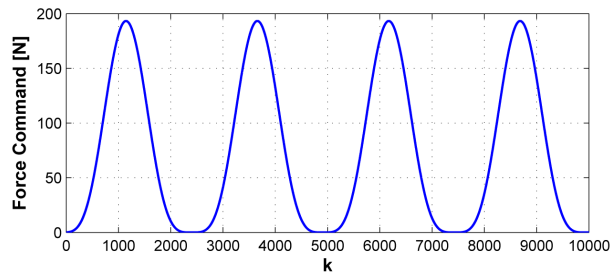
Figure 10. Force command.
