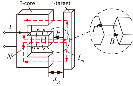
Figure 2. Sketches of the E-core actuator.
