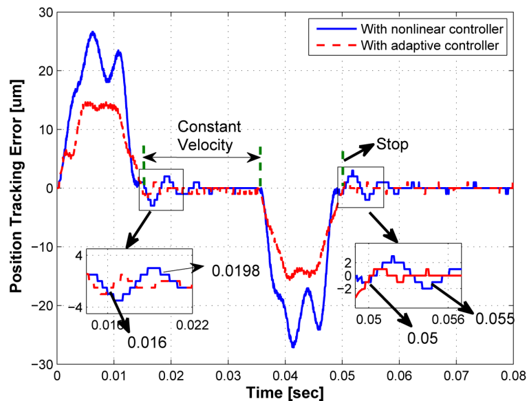
Figure 12. Comparison of the position tracking error between with nonlinear compensator and with adaptive MNN controller.
