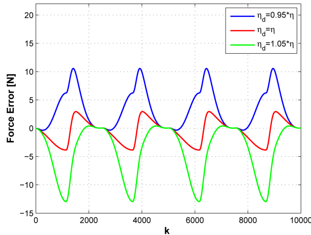
Figure 7. Force error with nonlinear compensator.
