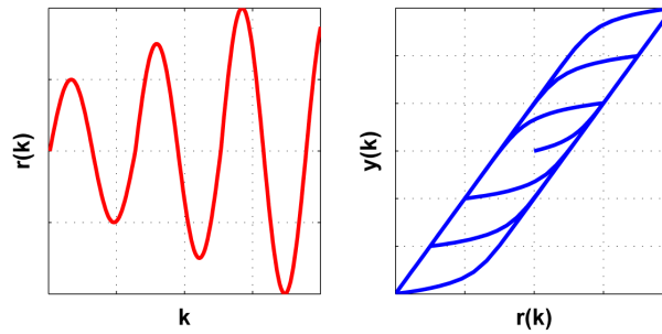
Figure 1. Input r(k) (left) and the corresponding output y(k) map (right) trajectories of the parametric hysteresis operator.
