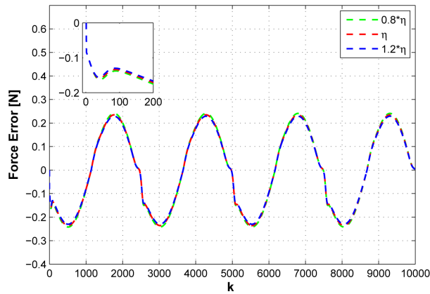
Figure 8. Force error with adaptive MNN controller.
