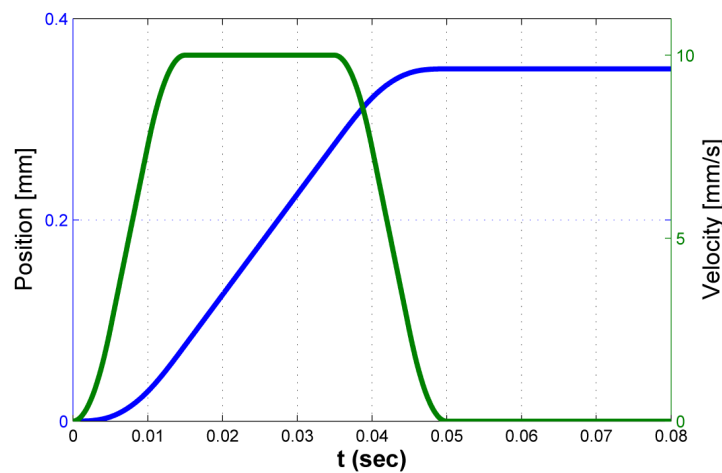
Figure 11. Reference position and velocity.
