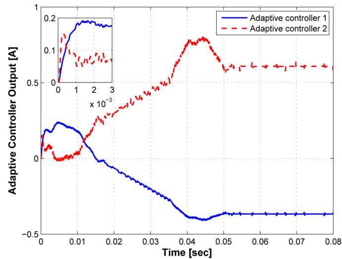
Figure 13. Outputs of the adaptive controllers.
