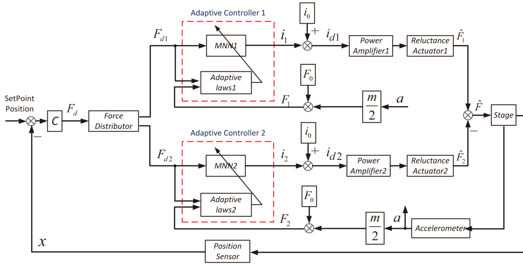
Figure 6. Nonlinear control structure for stage having paired E/I core actuator using adaptive MNN.
