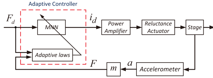
Figure 4. Direct adaptive MNN control for reluctance linear actuator.
