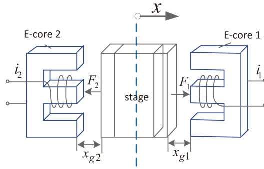
Figure 5. Paired E/I core actuator.
