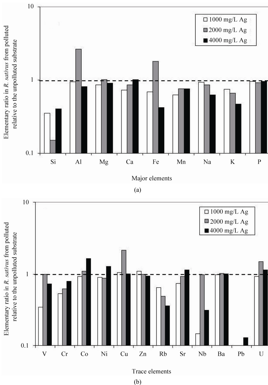
Figure 1. (a) Ratios among the major-element concentrations in Raphanus sativus from \text{AgNO}_3 polluted substrates relative to the same elements in the species from unpolluted substrate; (b) Ratios among the trace-element concentrations in Raphanus sativus from \text{AgNO}_3 polluted substrates relative to the same elements in the species from unpolluted substrate. In both cases, an identical uptake is shown by a ratio of 1.
