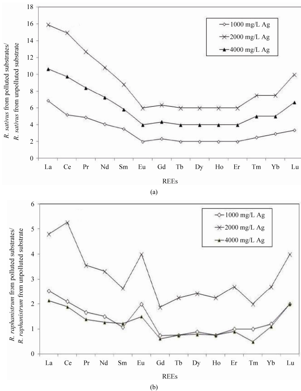
Figure 4. (a) REE composition of Raphanus sativus from the \text{AgNO}_3 polluted substrates normalized to the REE concentrations in the same species from unpolluted substrate; (b) REE composition of Raphanus raphanistrum from the \text{AgNO}_3 polluted substrate normalized to the REE concentrations in the same species from unpolluted substrate.
