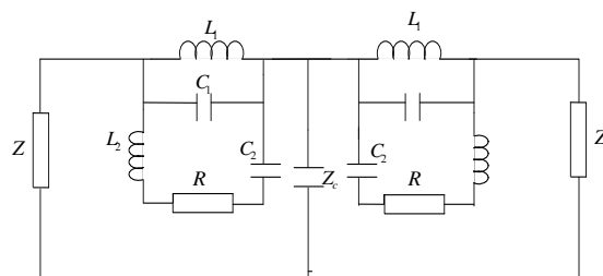
Figure 3. Equivalent circuit.
