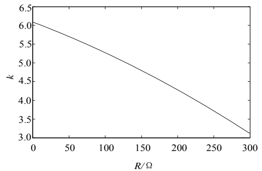
Figure 6. k change with the change of the transition resistance.
